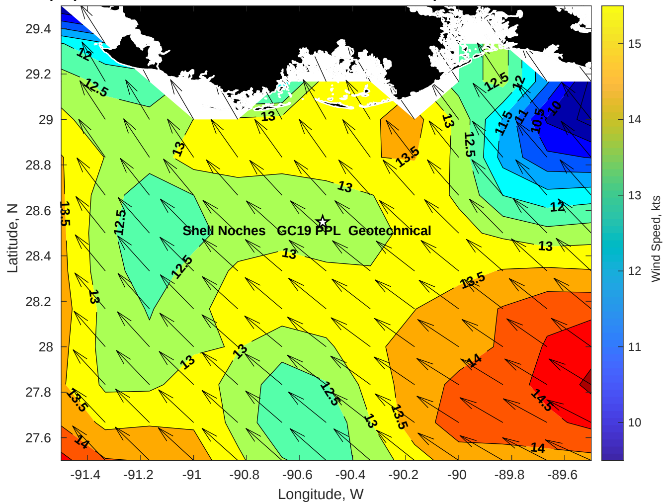
Winds (kts) for Shell Noches GC19 PPL Geotechnical at 29-Apr-2025 09:00:00
