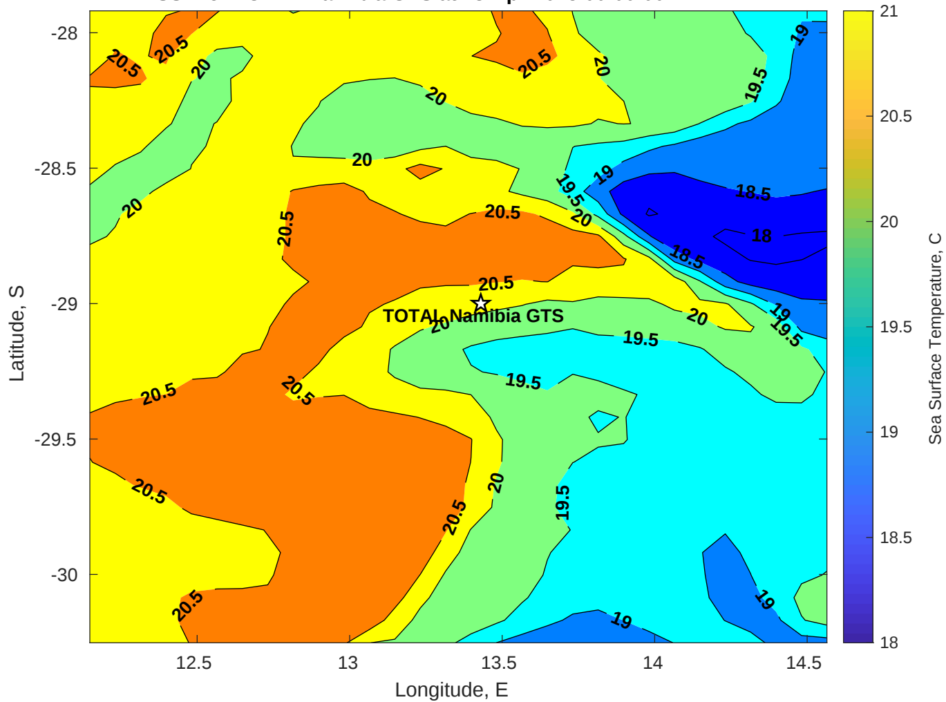
SST for TOTAL Namibia GTS at 28-Apr-2025 00:00:00
