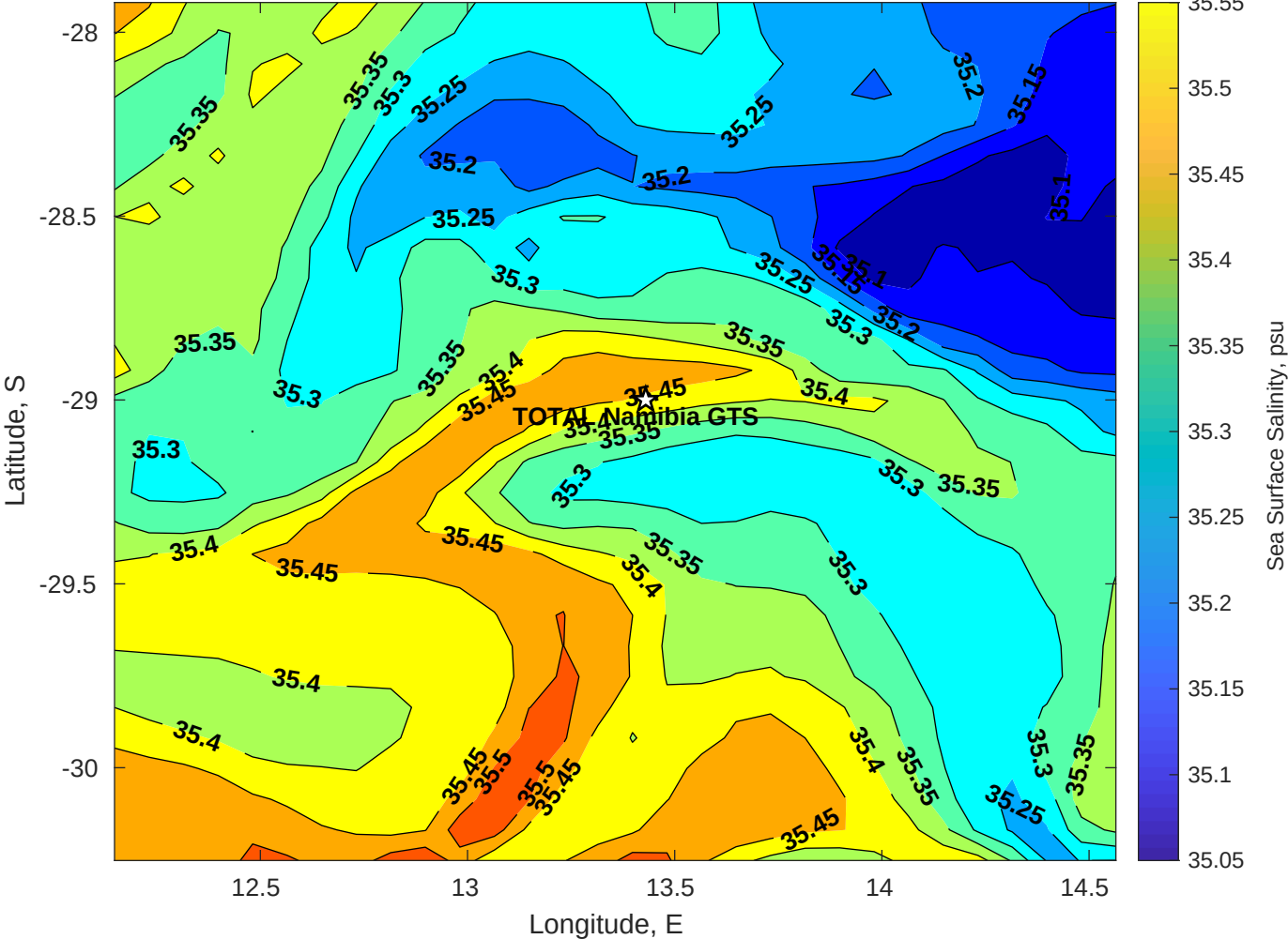
Surface Salinity for TOTAL Namibia GTS at 28-Apr-2025 00:00:00
