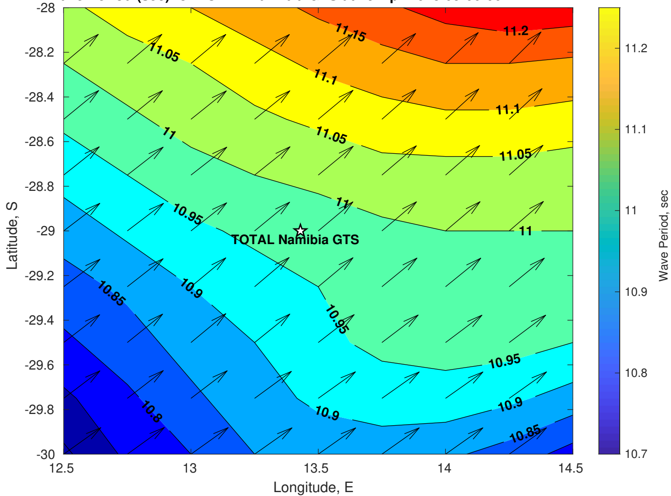
Wave Period (sec) for TOTAL Namibia GTS at 29-Apr-2025 09:00:00
