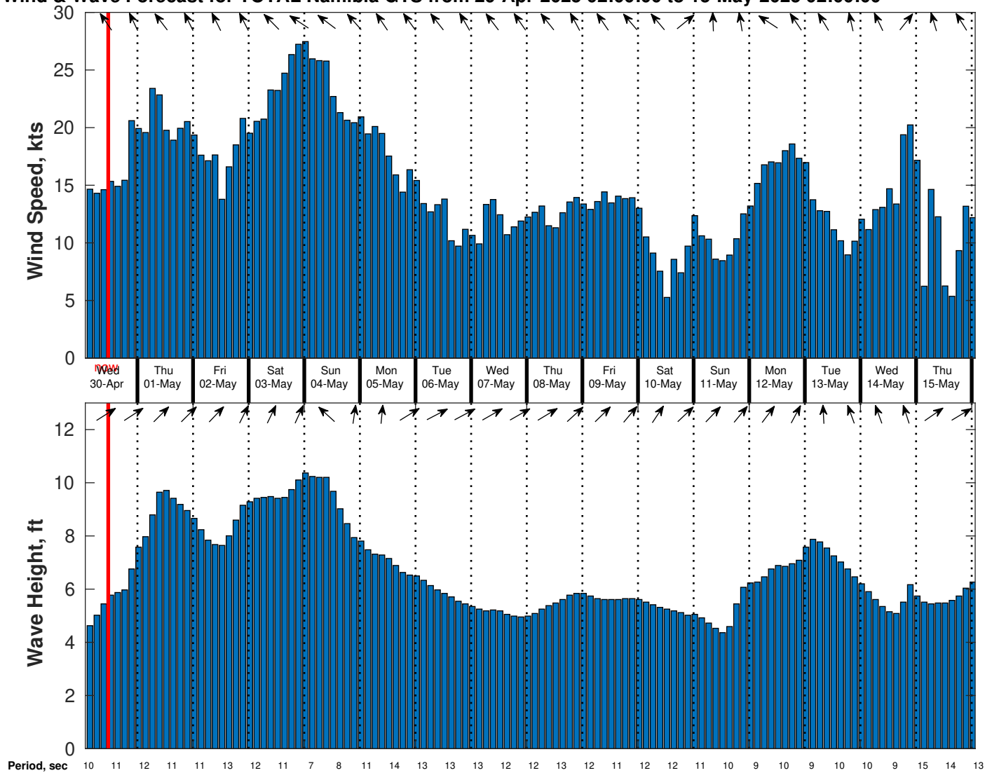
Wind & Wave Forecast for TOTAL Namibia GTS from 29-Apr-2025 02:00:00 to 15-May-2025 02:00:00
