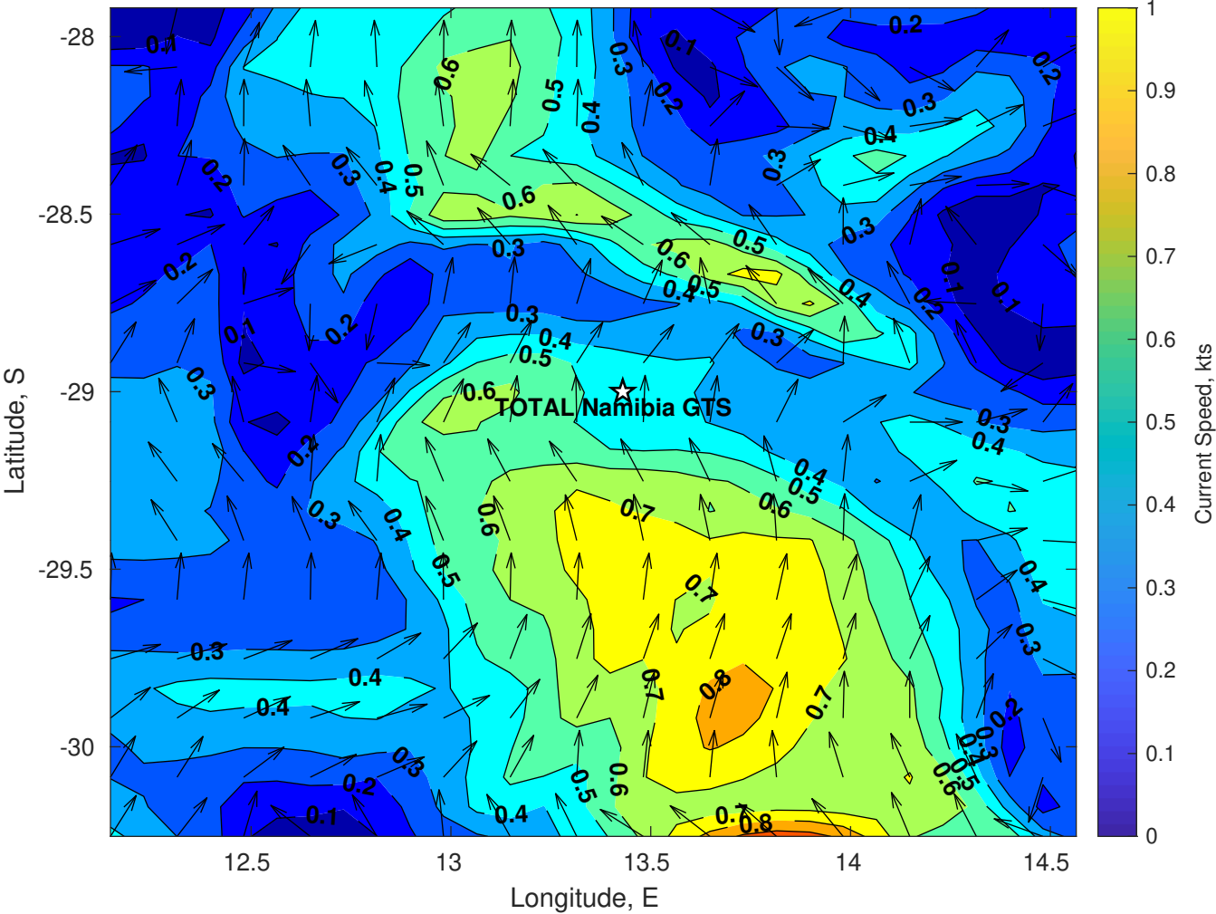
Surface Currents for TOTAL Namibia GTS at 28-Apr-2025 00:00:00
