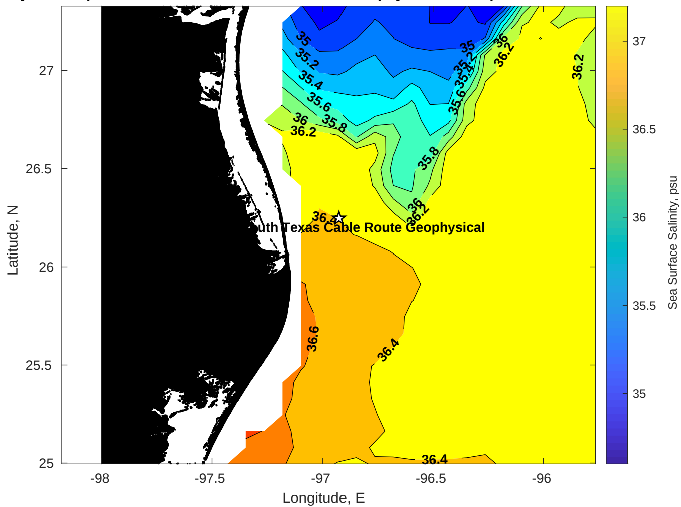
Surface Salinity for Tampnet P2378 South Texas Cable Route Geophysical at 28-Apr-2025 00:00:00
