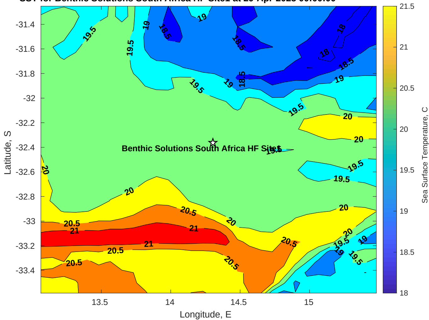
SST for Benthic Solutions South Africa HF Site1 at 29-Apr-2025 00:00:00
