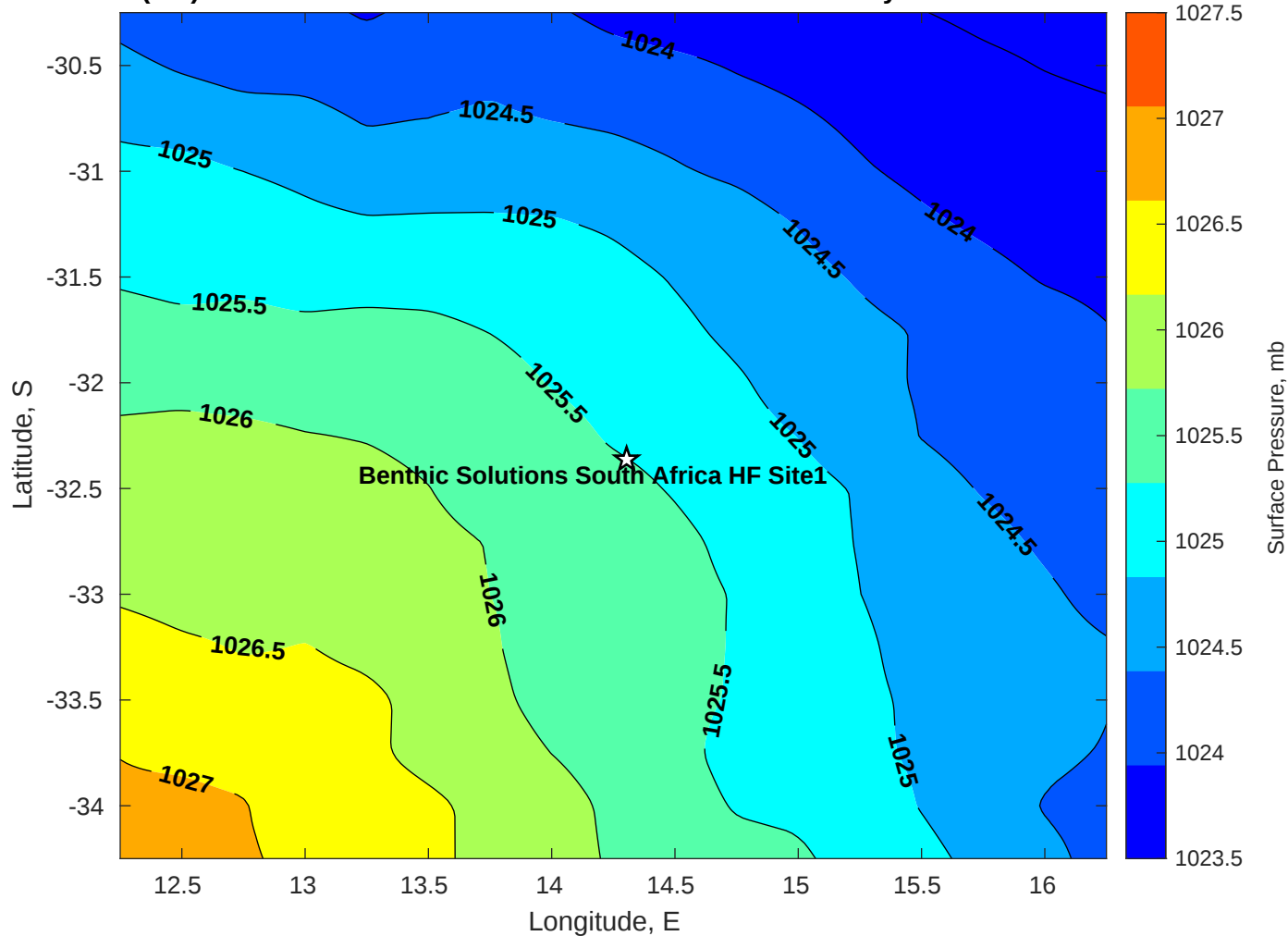
Surface Pressure (mb) for Benthic Solutions South Africa HF Site1 at 02-May-2025 00:00:00
