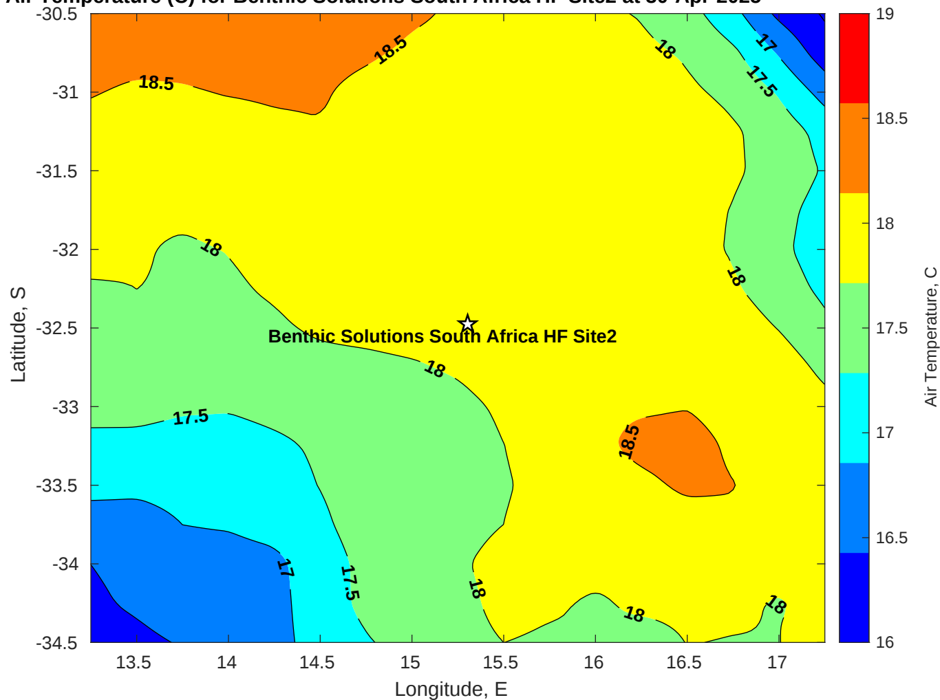
Air Temperature (C) for Benthic Solutions South Africa HF Site2 at 30-Apr-2025
