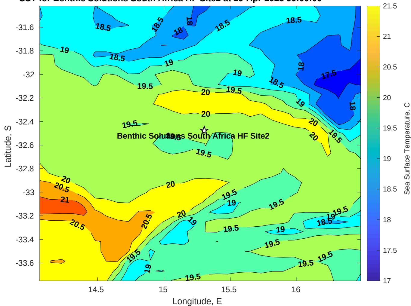
SST for Benthic Solutions South Africa HF Site2 at 29-Apr-2025 00:00:00
