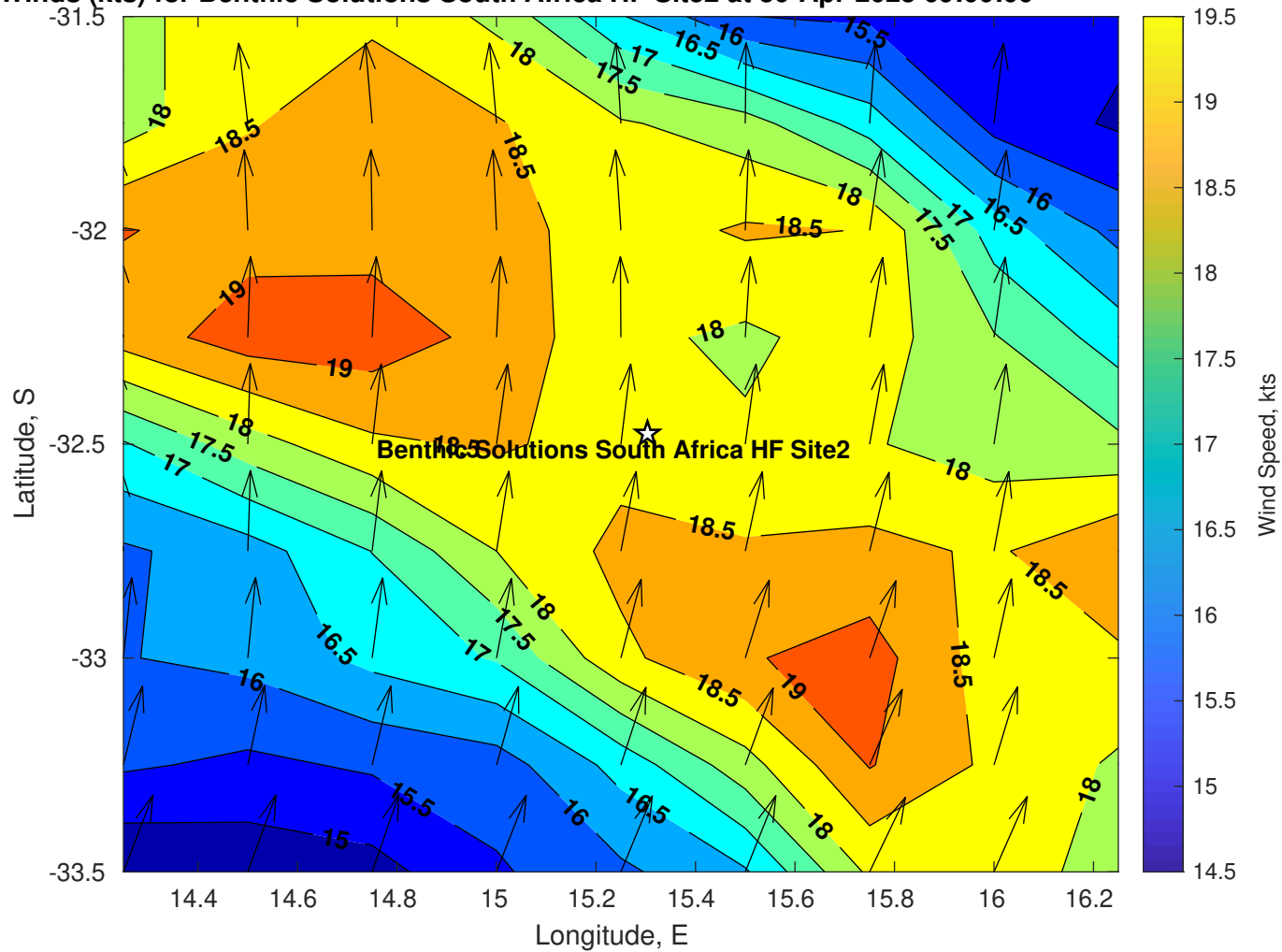
Winds (kts) for Benthic Solutions South Africa HF Site2 at 30-Apr-2025 09:00:00
