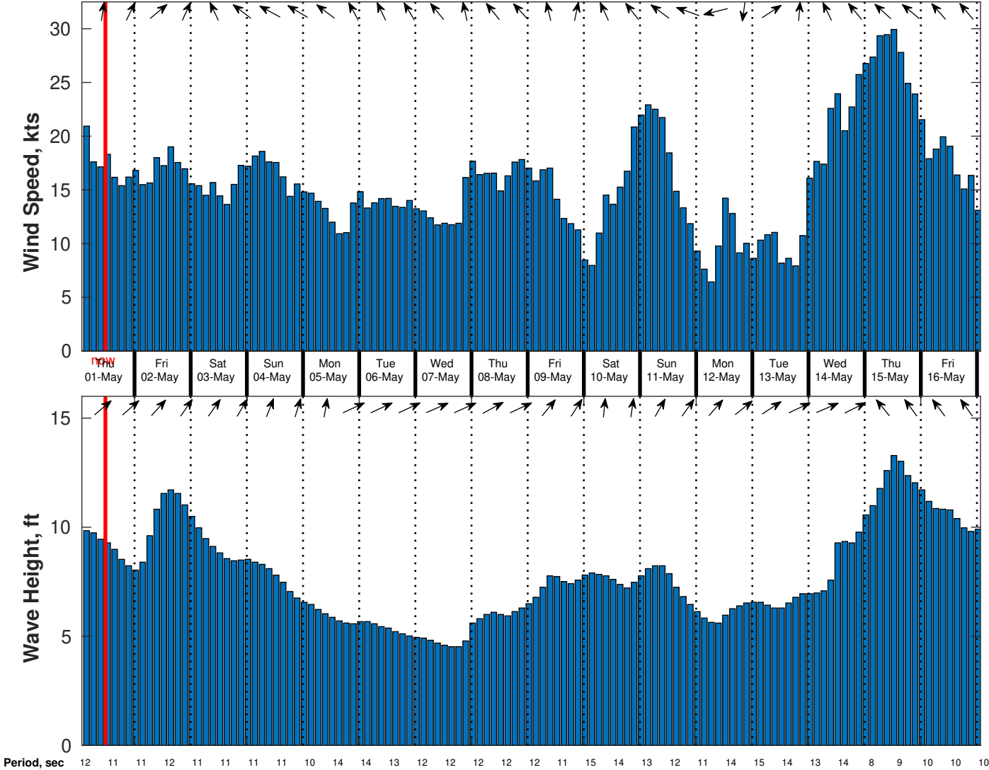
Wind & Wave Forecast for Benthic Solutions South Africa HF Site2 from 30-Apr-2025 02:00:00 to 16-May-2025 02:00:00
