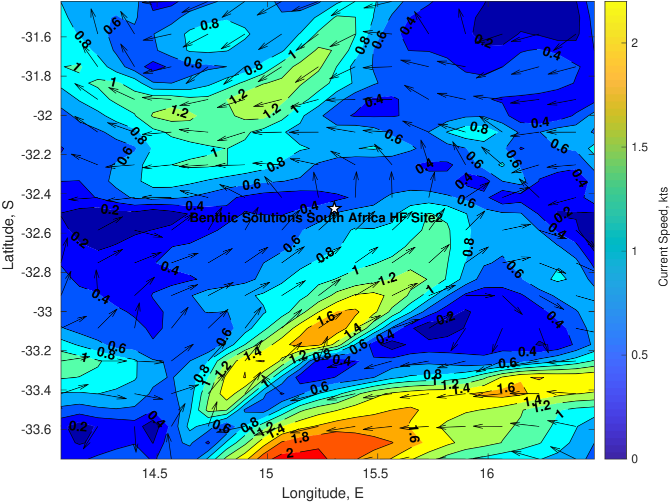
Surface Currents for Benthic Solutions South Africa HF Site2 at 29-Apr-2025 00:00:00
