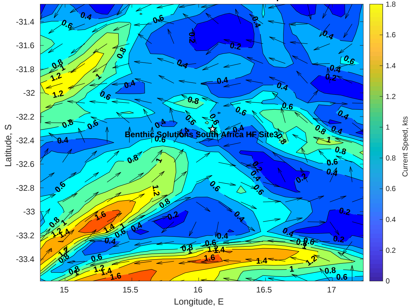
Surface Currents for Benthic Solutions South Africa HF Site3 at 29-Apr-2025 00:00:00
