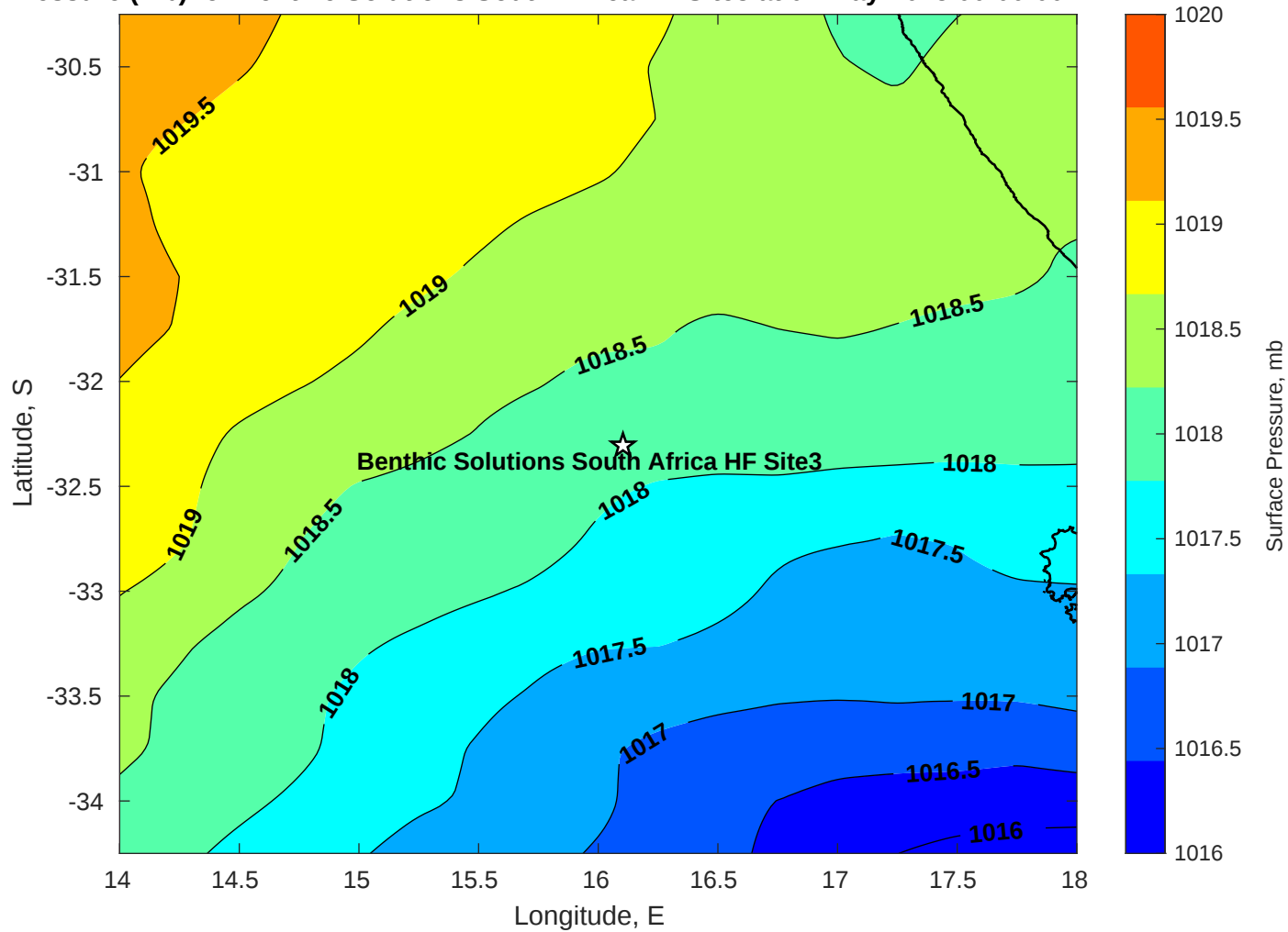
Surface Pressure (mb) for Benthic Solutions South Africa HF Site3 at 01-May-2025 00:00:00
