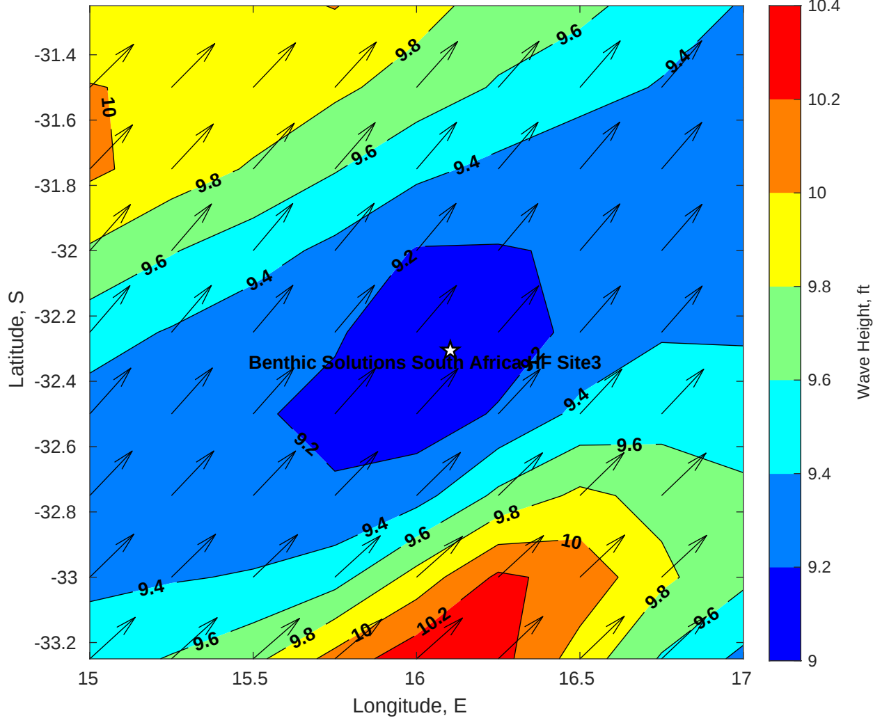
Wave Height (ft) for Benthic Solutions South Africa HF Site3 at 30-Apr-2025 09:00:00
