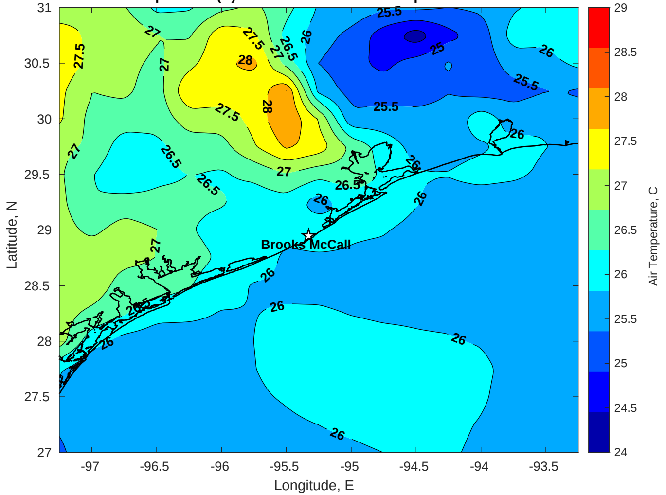
Air Temperature (C) for Brooks McCall at 30-Apr-2025
