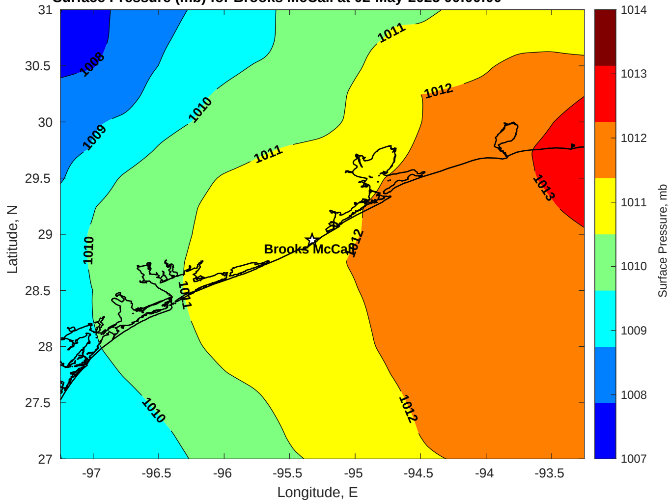
Surface Pressure (mb) for Brooks McCall at 02-May-2025 00:00:00
