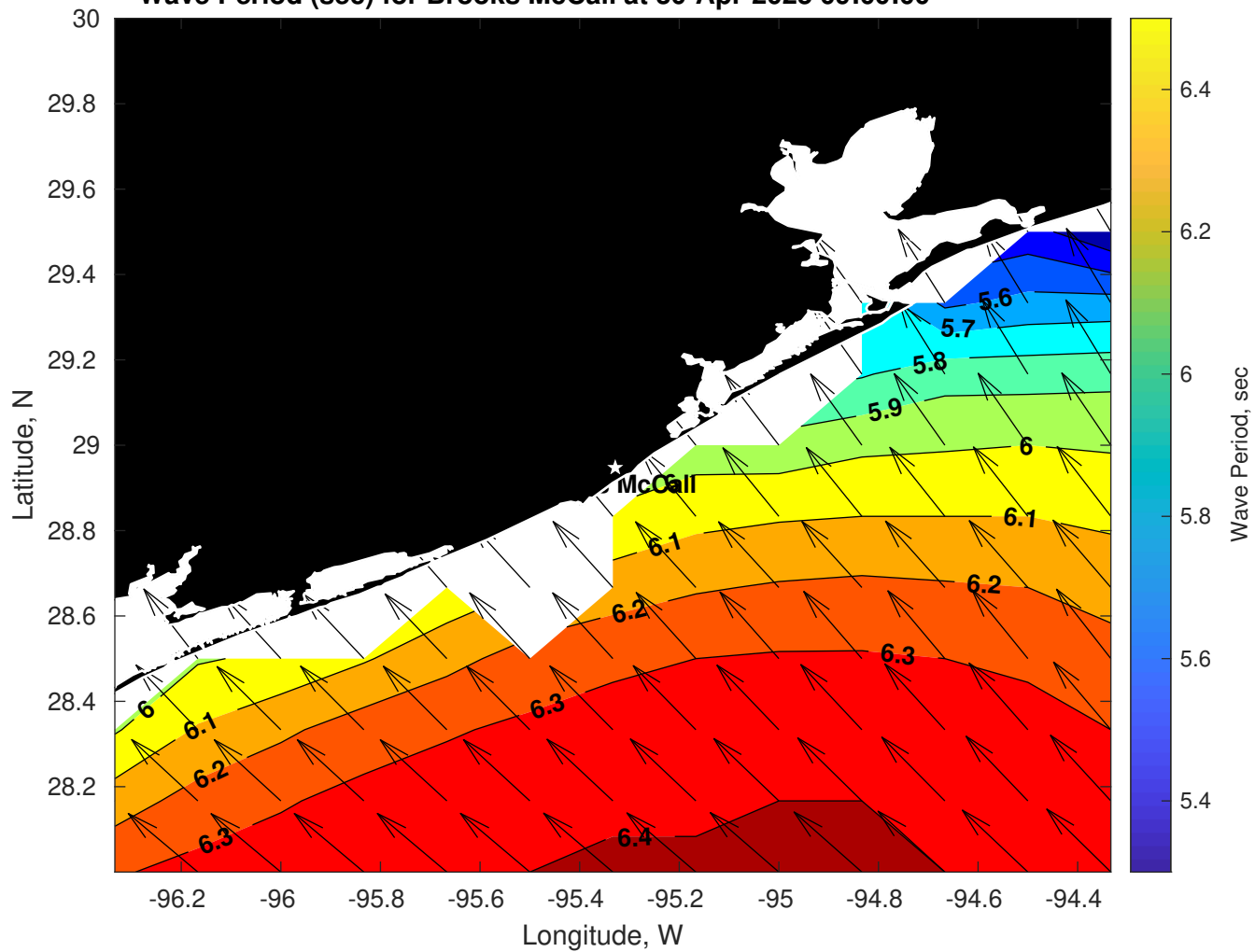
Wave Period (sec) for Brooks McCall at 30-Apr-2025 09:00:00
