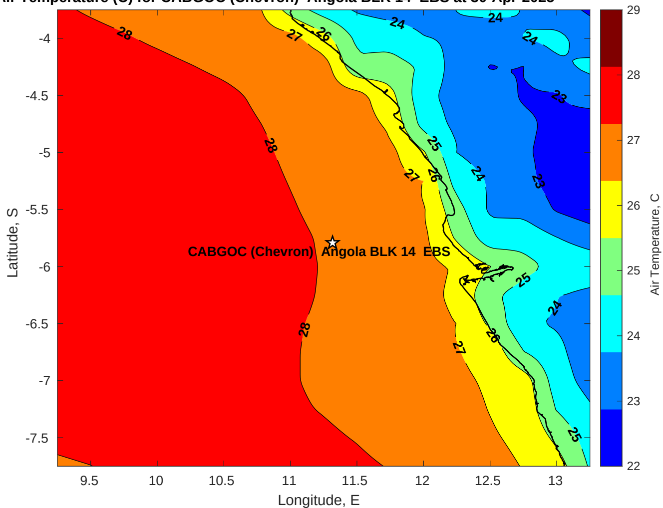
Air Temperature (C) for CABGOC (Chevron) Angola BLK 14 EBS at 30-Apr-2025
