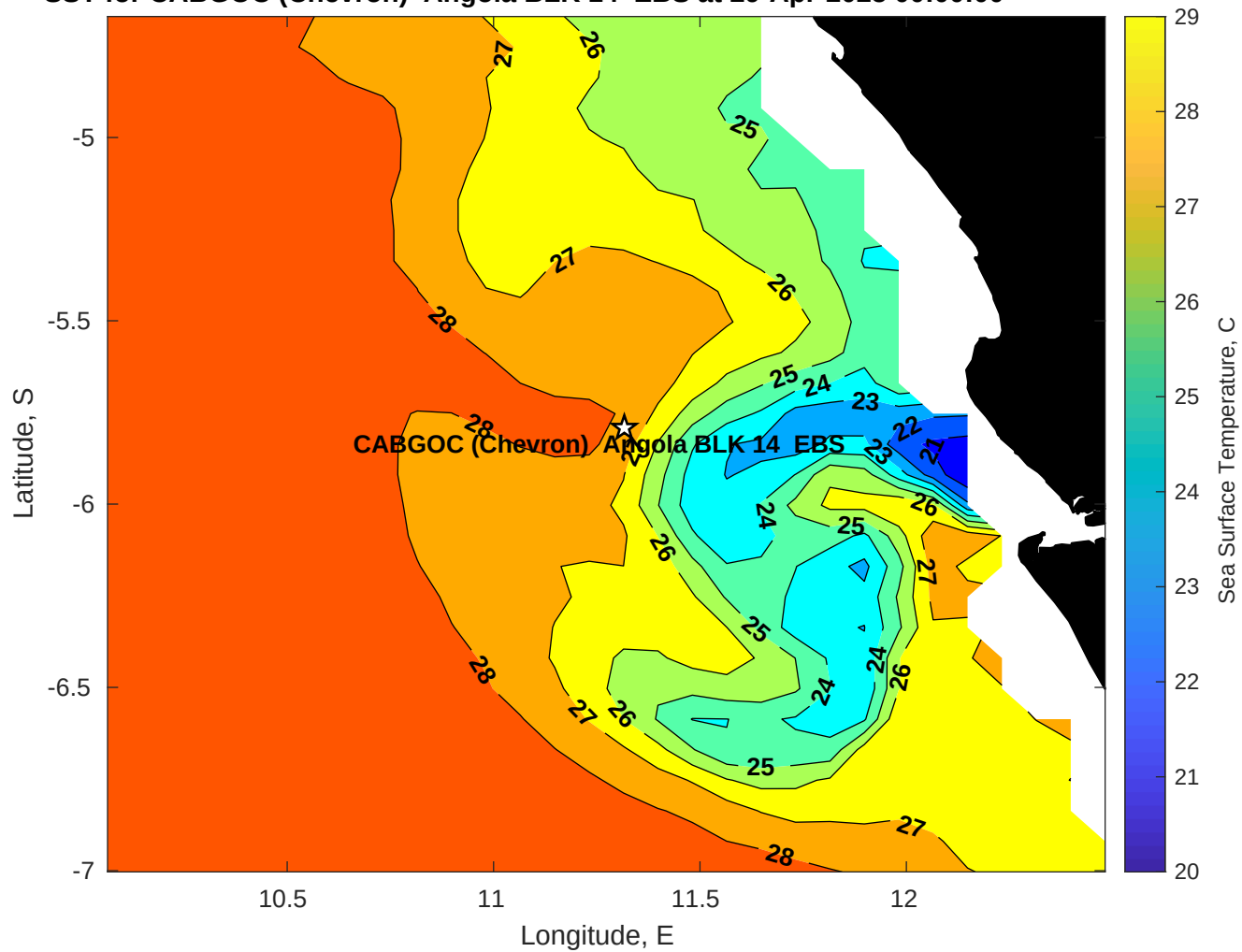
SST for CABGOC (Chevron) Angola BLK 14 EBS at 29-Apr-2025 00:00:00
