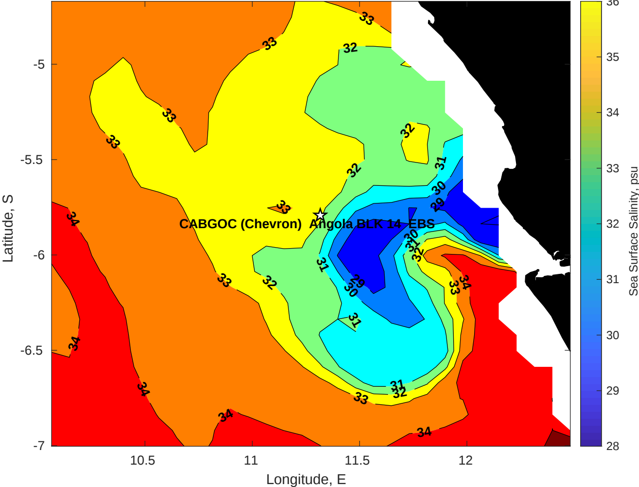
Surface Salinity for CABGOC (Chevron) Angola BLK 14 EBS at 29-Apr-2025 00:00:00
