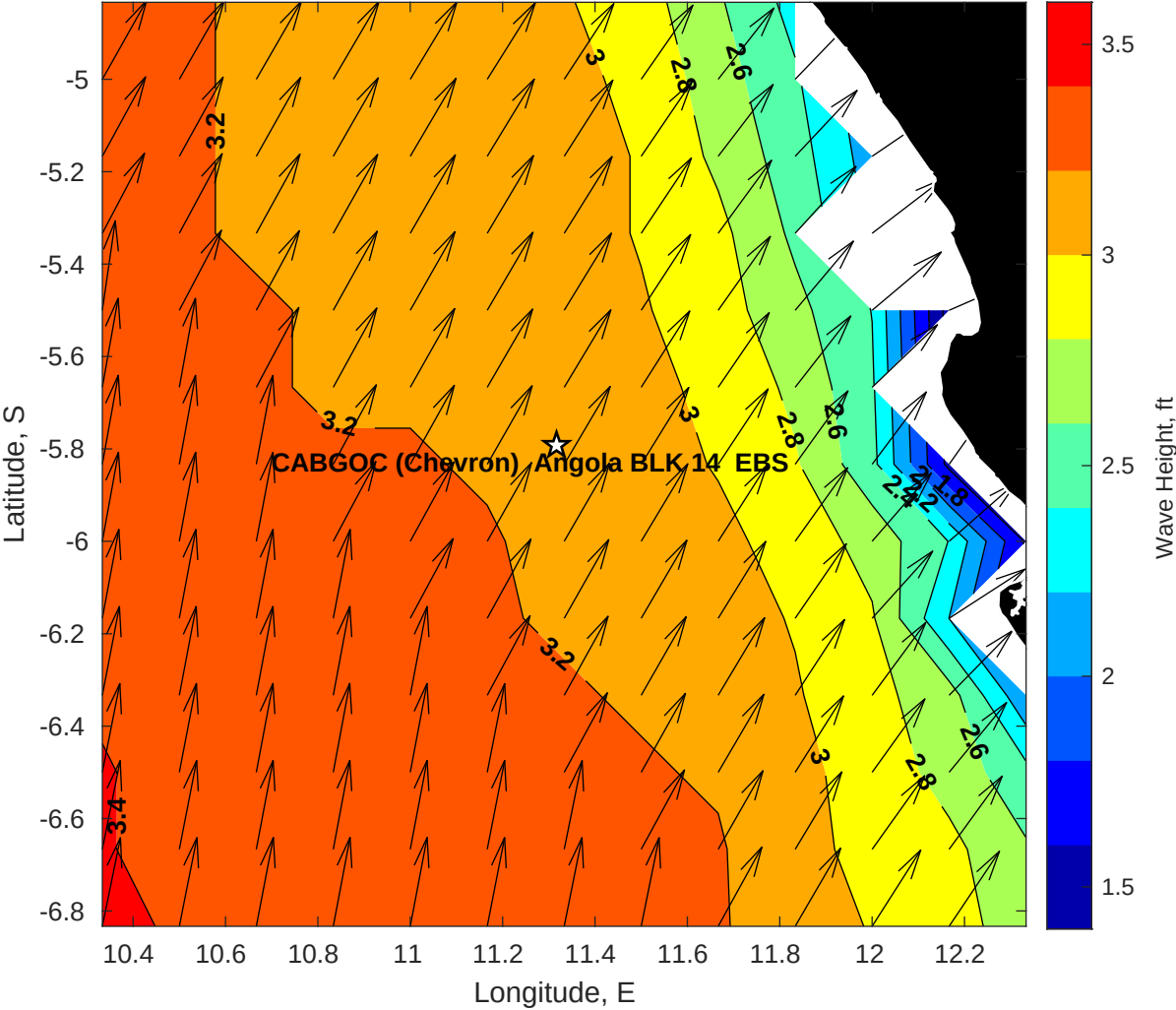
Wave Height (ft) for CABGOC (Chevron) Angola BLK 14 EBS at 30-Apr-2025 09:00:00
