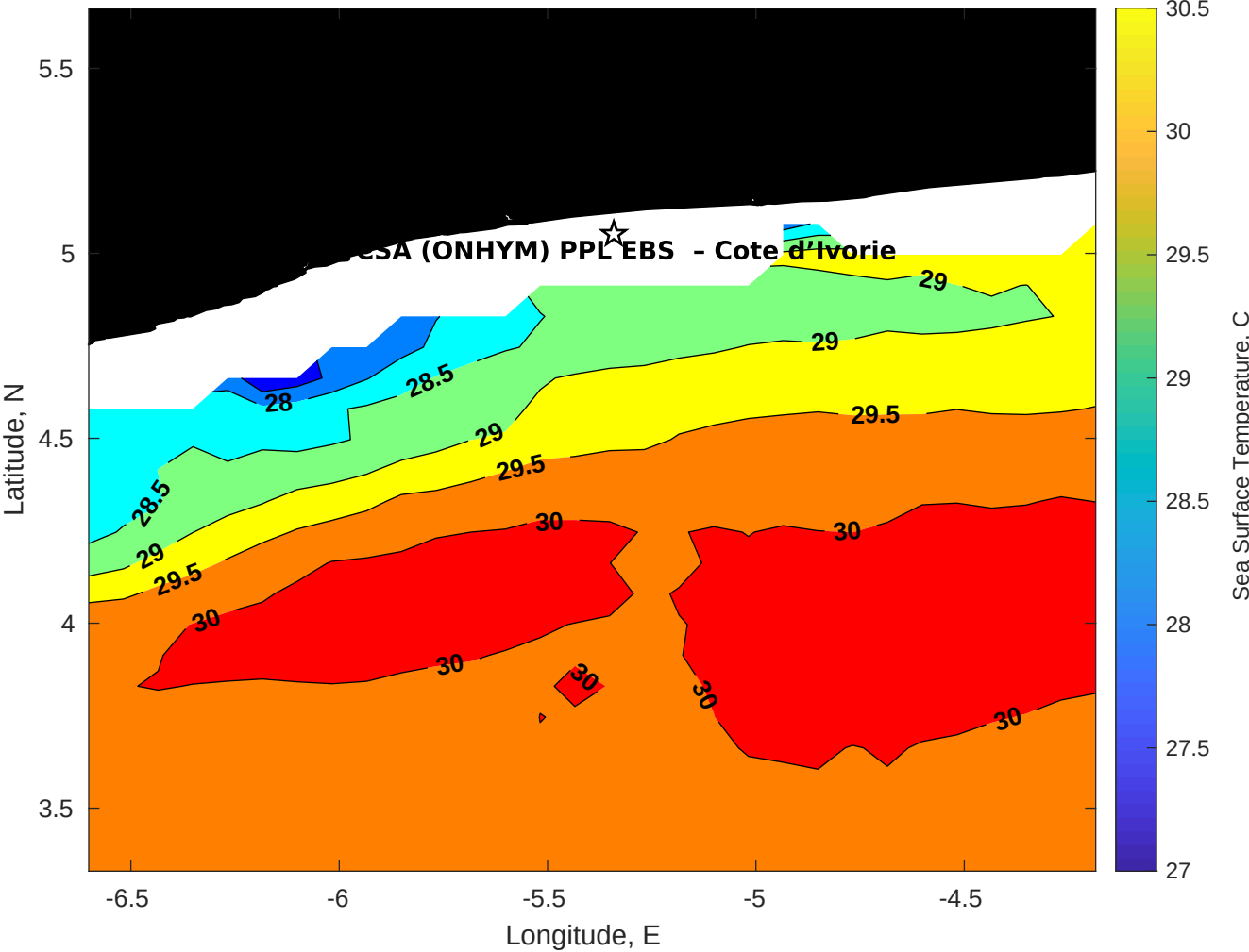
SST for CSA (ONHYM) PPL EBS - Cote d'Ivoire at 29-Apr-2025 00:00:00
