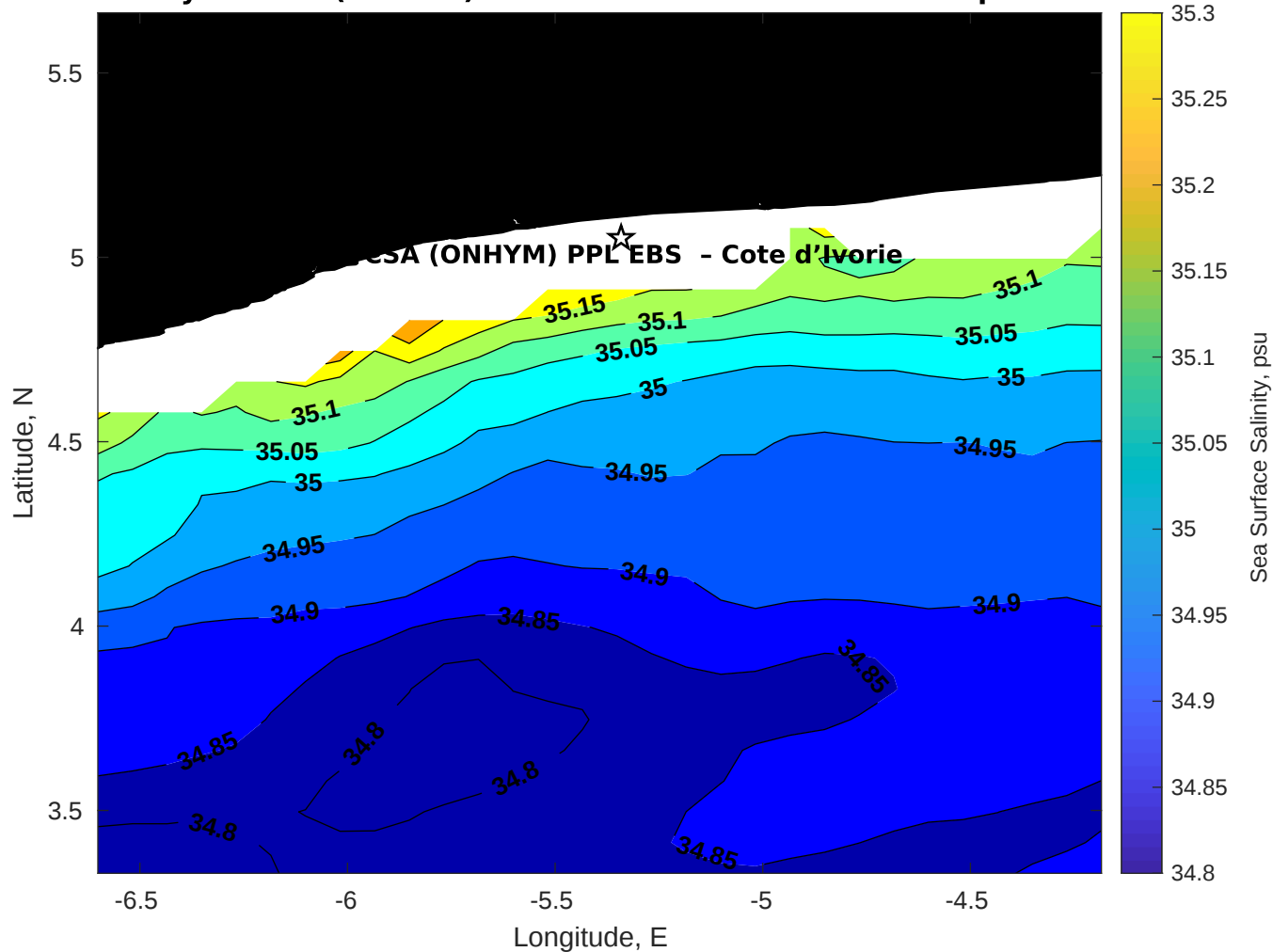
Surface Salinity for CSA (ONHYM) PPL EBS - Cote d'Ivoire at 29-Apr-2025 00:00:00
