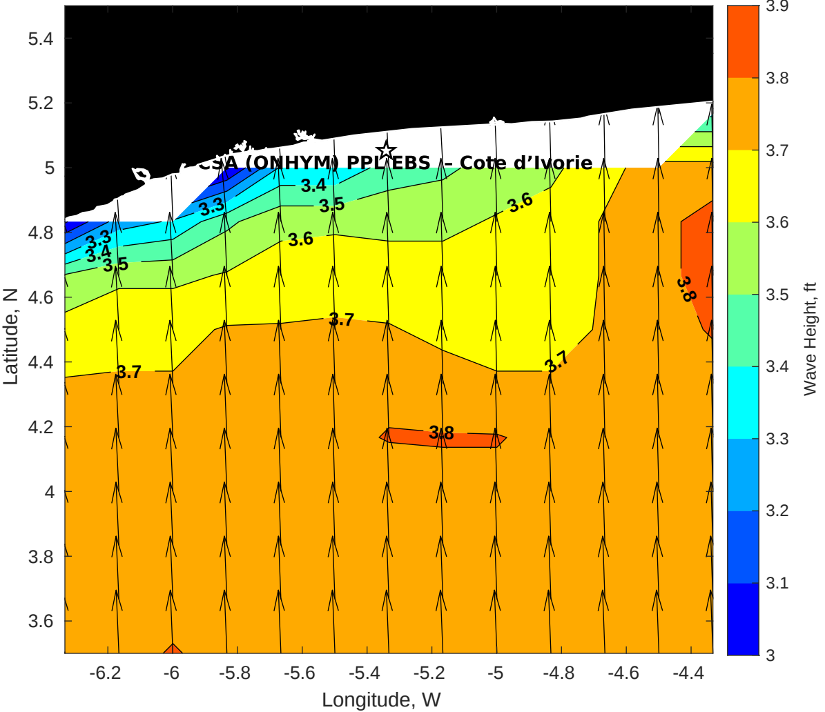
Wave Height (ft) for CSA (ONHYM) PPL EBS - Cote d'Ivoire at 30-Apr-2025 09:00:00
