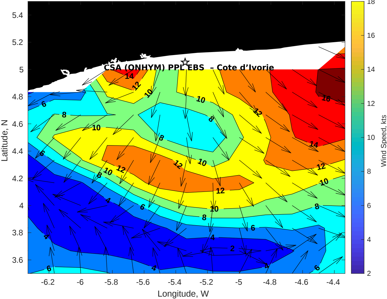
Winds (kts) for CSA (ONHYM) PPL EBS - Cote d'Ivoire at 30-Apr-2025 09:00:00
