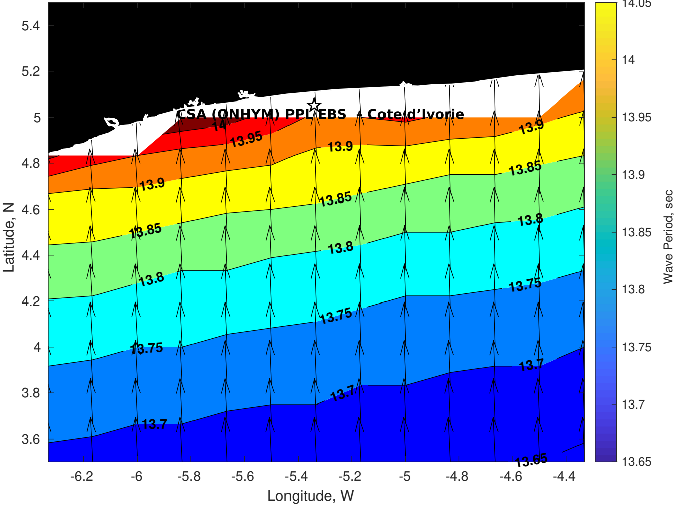
Wave Period (sec) for CSA (ONHYM) PPL EBS - Cote d'Ivoire at 30-Apr-2025 09:00:00
