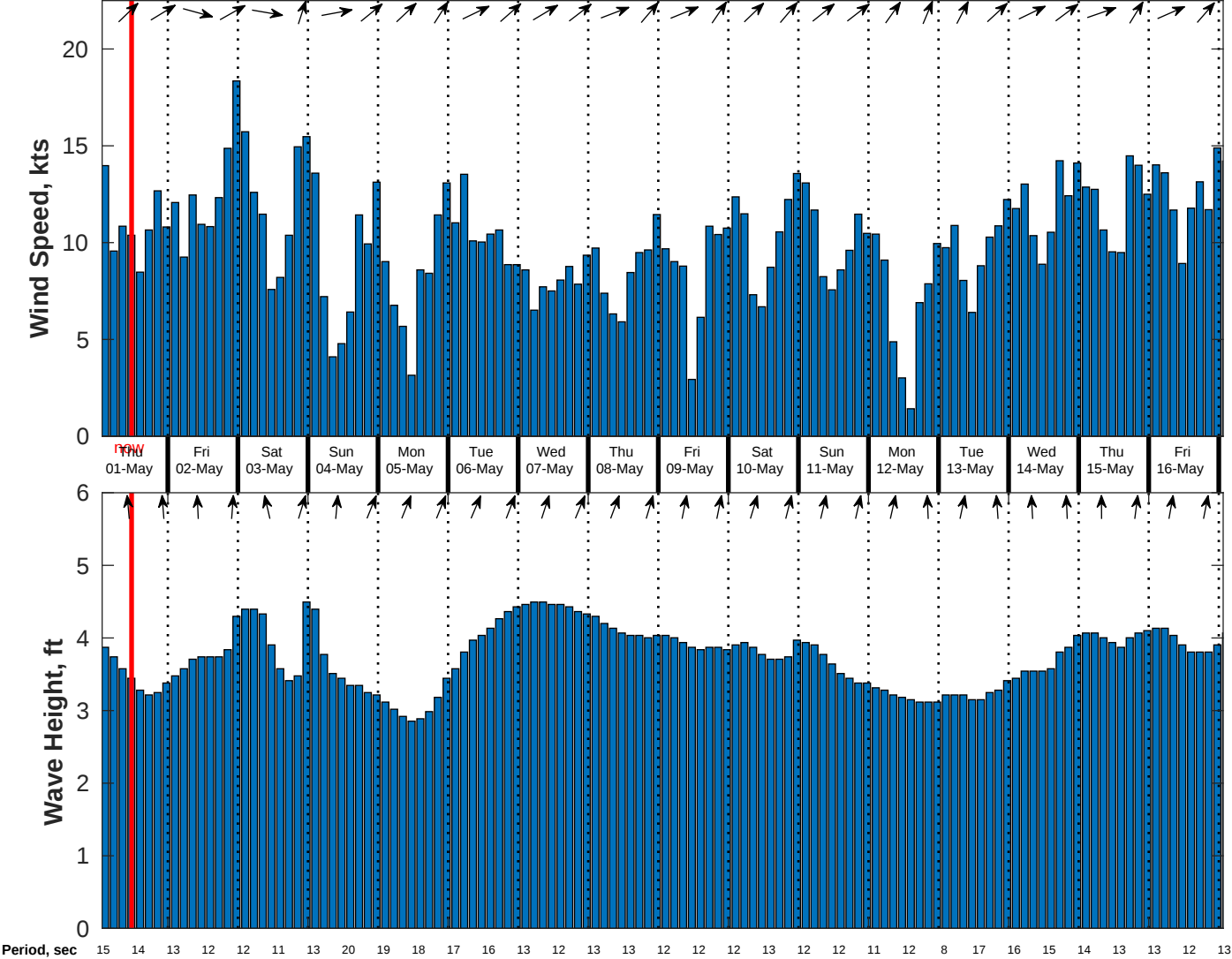
Wind & Wave Forecast for CSA (ONHYM) PPL EBS - Cote d'Ivoire from 30-Apr-2025 01:00:00 to 16-May-2025 01:00:00
