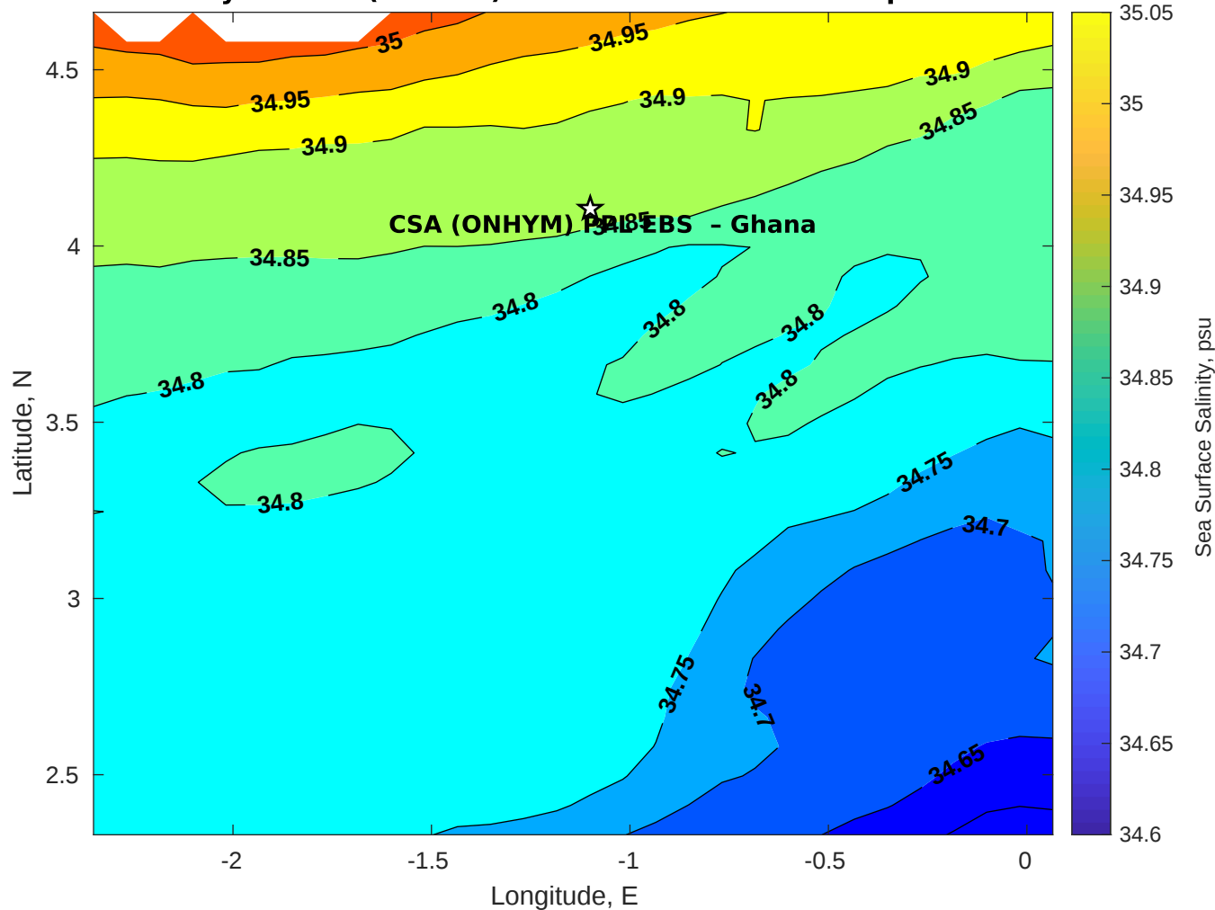
Surface Salinity for CSA (ONHYM) PPL EBS - Ghana at 29-Apr-2025 00:00:00
