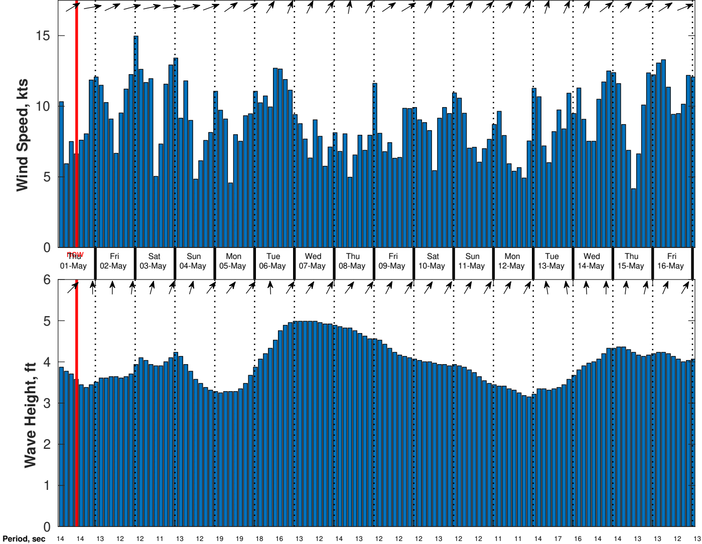
Wind & Wave Forecast for CSA (ONHYM) PPL EBS - Ghana from 30-Apr-2025 02:00:00 to 16-May-2025 02:00:00
