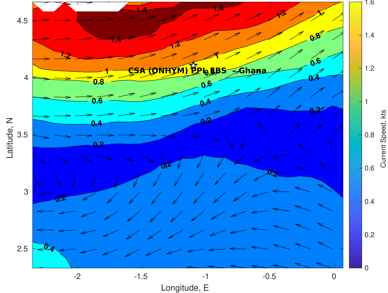
Surface Currents for CSA (ONHYM) PPL EBS - Ghana at 29-Apr-2025 00:00:00
