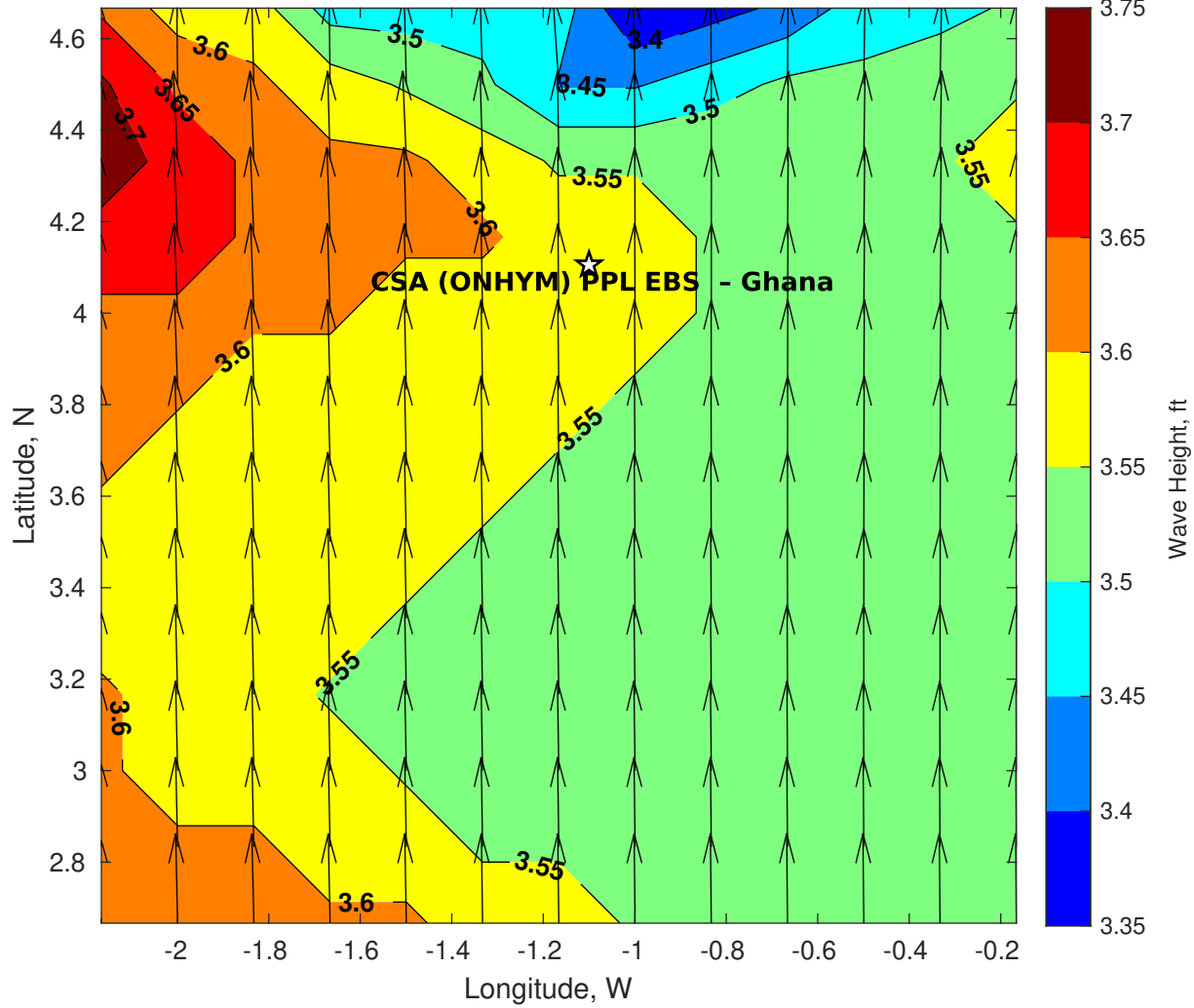
Wave Height (ft) for CSA (ONHYM) PPL EBS - Ghana at 30-Apr-2025 09:00:00
