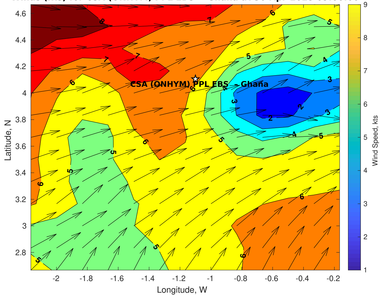
Winds (kts) for CSA (ONHYM) PPL EBS - Ghana at 30-Apr-2025 09:00:00
