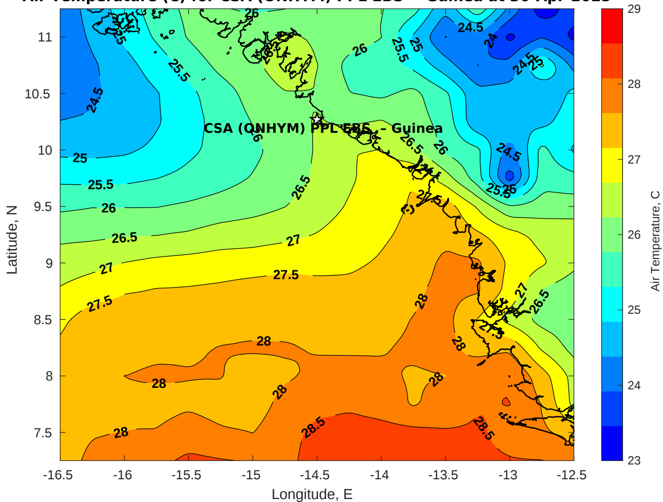
Air Temperature (C) for CSA (ONHYM) PPL EBS - Guinea at 30-Apr-2025
