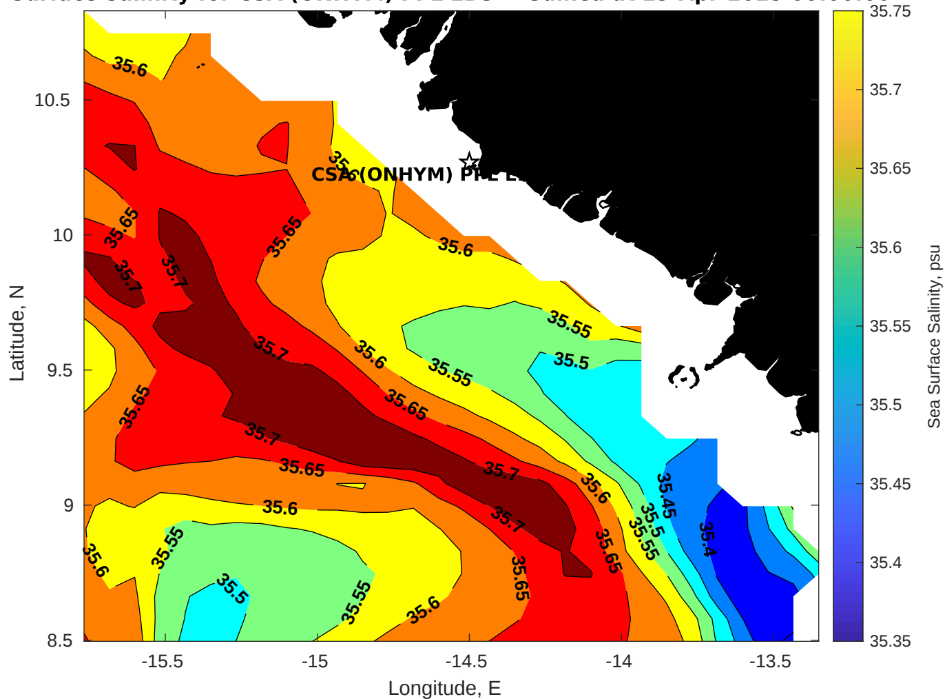
Surface Salinity for CSA (ONHYM) PPL EBS - Guinea at 29-Apr-2025 00:00:00
