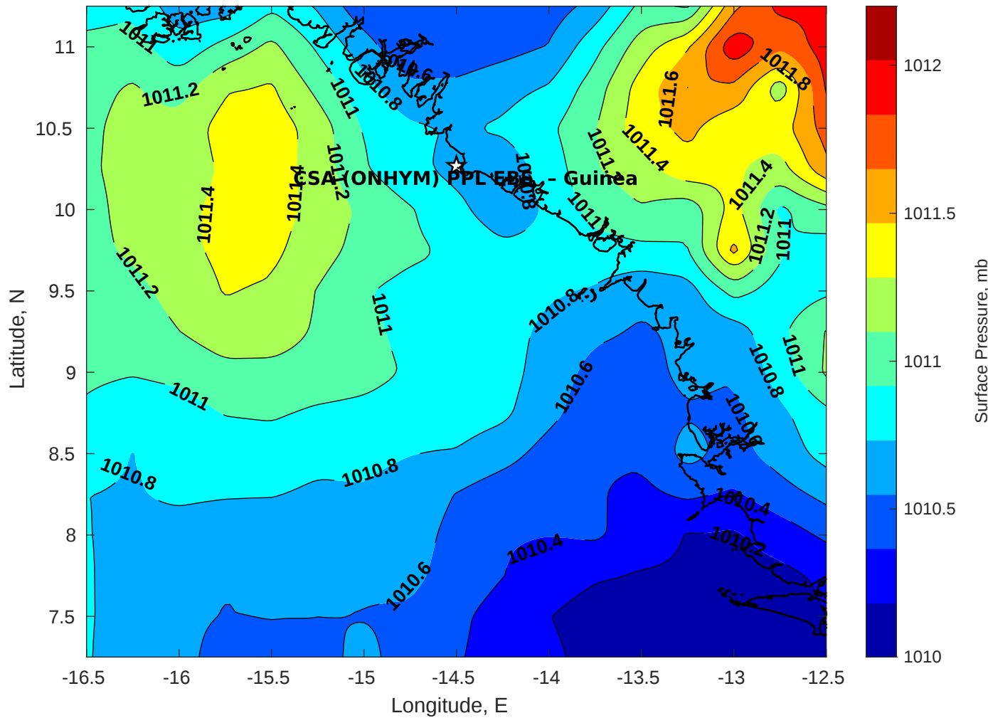
Surface Pressure (mb) for CSA (ONHYM) PPL EBS - Guinea at 30-Apr-2025 00:00:00
