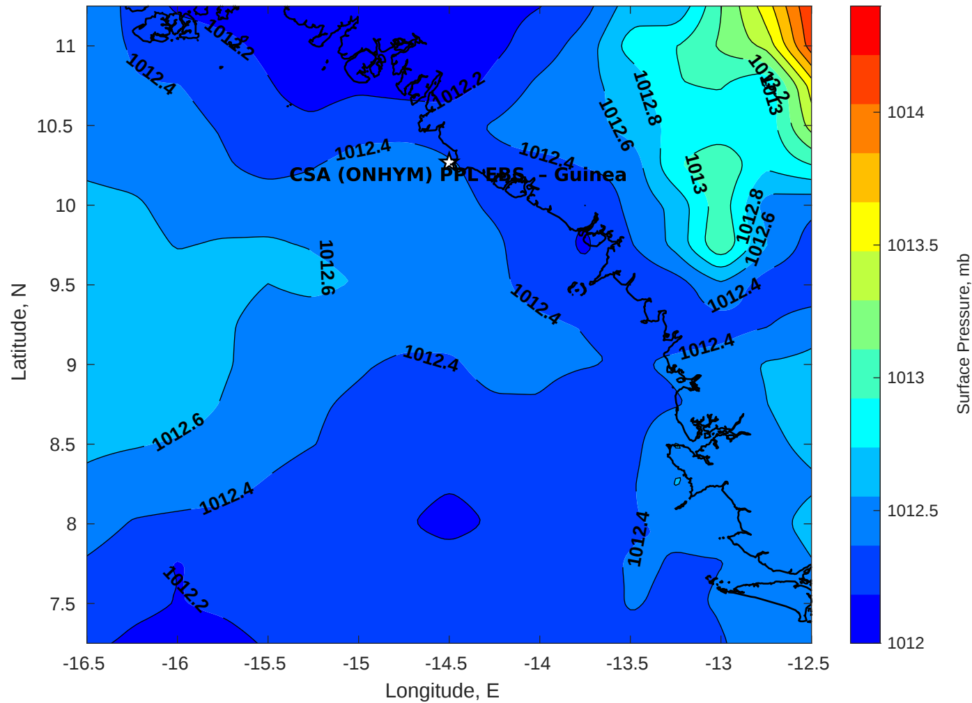
Surface Pressure (mb) for CSA (ONHYM) PPL EBS - Guinea at 02-May-2025 00:00:00
