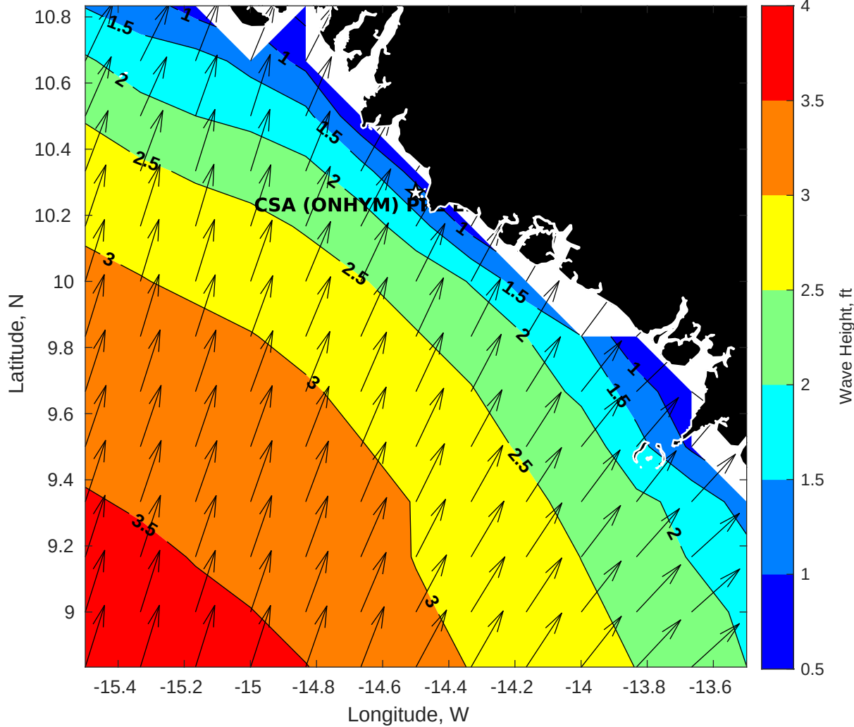
Wave Height (ft) for CSA (ONHYM) PPL EBS - Guinea at 30-Apr-2025 09:00:00
