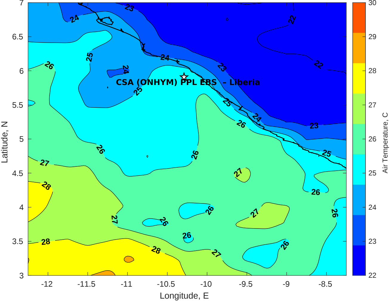
Air Temperature (C) for CSA (ONHYM) PPL EBS - Liberia at 30-Apr-2025
