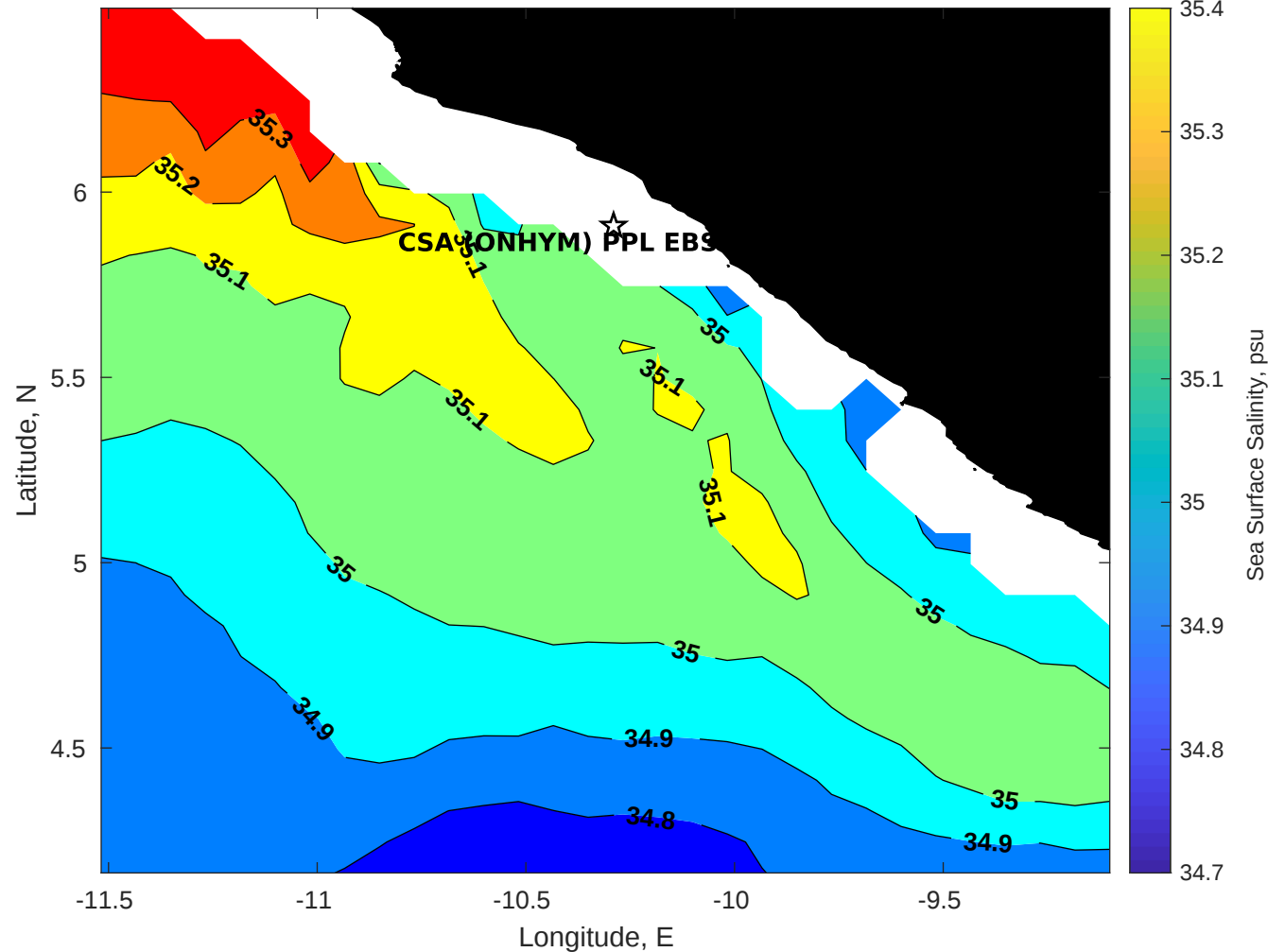
Surface Salinity for CSA (ONHYM) PPL EBS - Liberia at 29-Apr-2025 00:00:00
