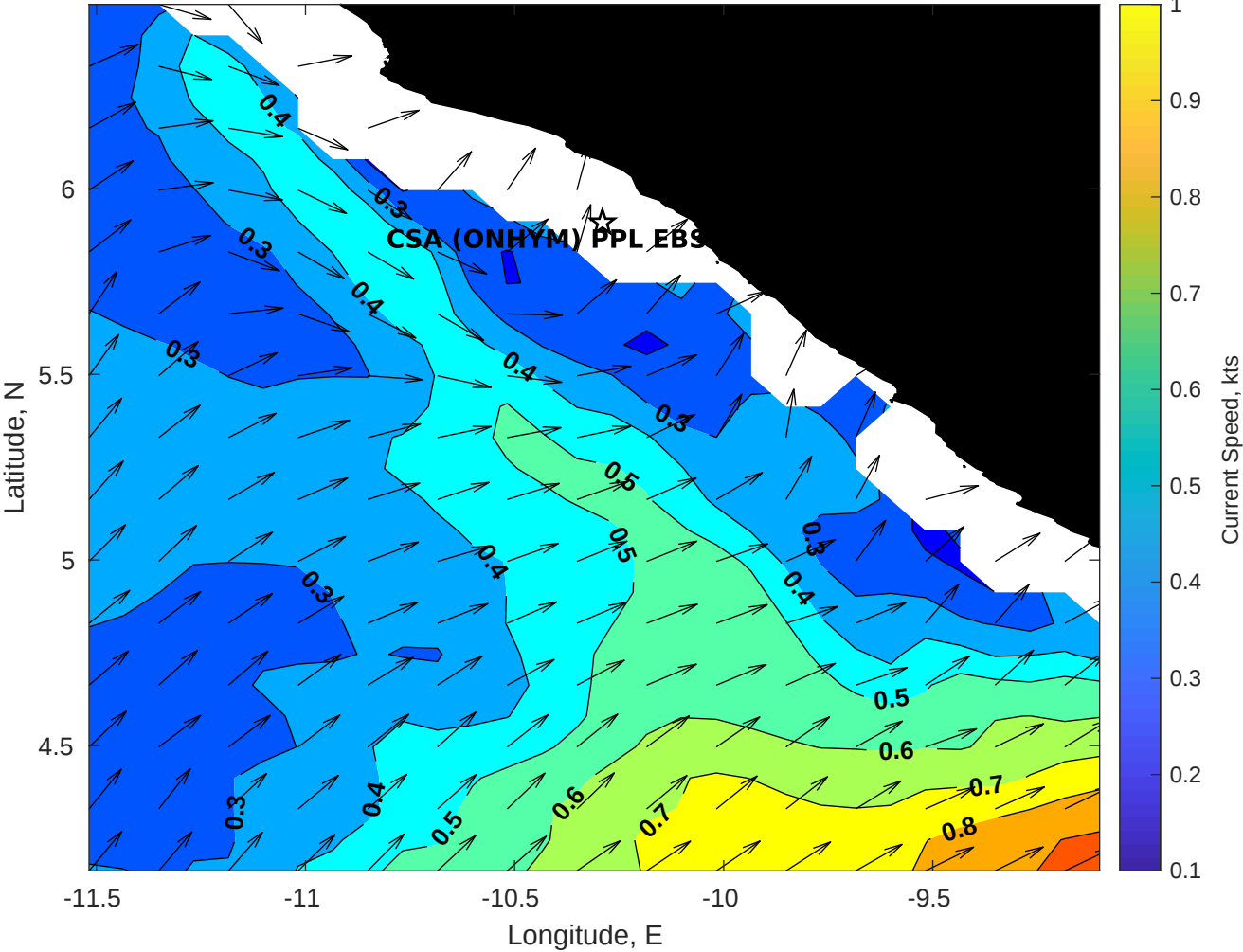
Surface Currents for CSA (ONHYM) PPL EBS - Liberia at 29-Apr-2025 00:00:00
