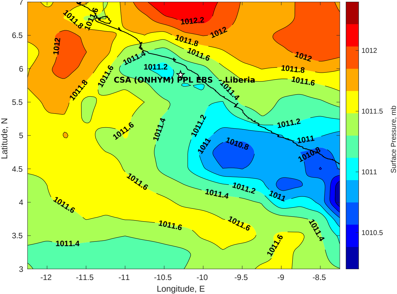
Surface Pressure (mb) for CSA (ONHYM) PPL EBS - Liberia at 01-May-2025 00:00:00
