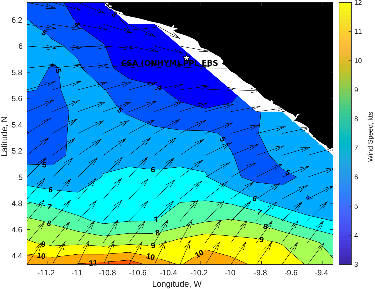
Winds (kts) for CSA (ONHYM) PPL EBS - Liberia at 30-Apr-2025 09:00:00
