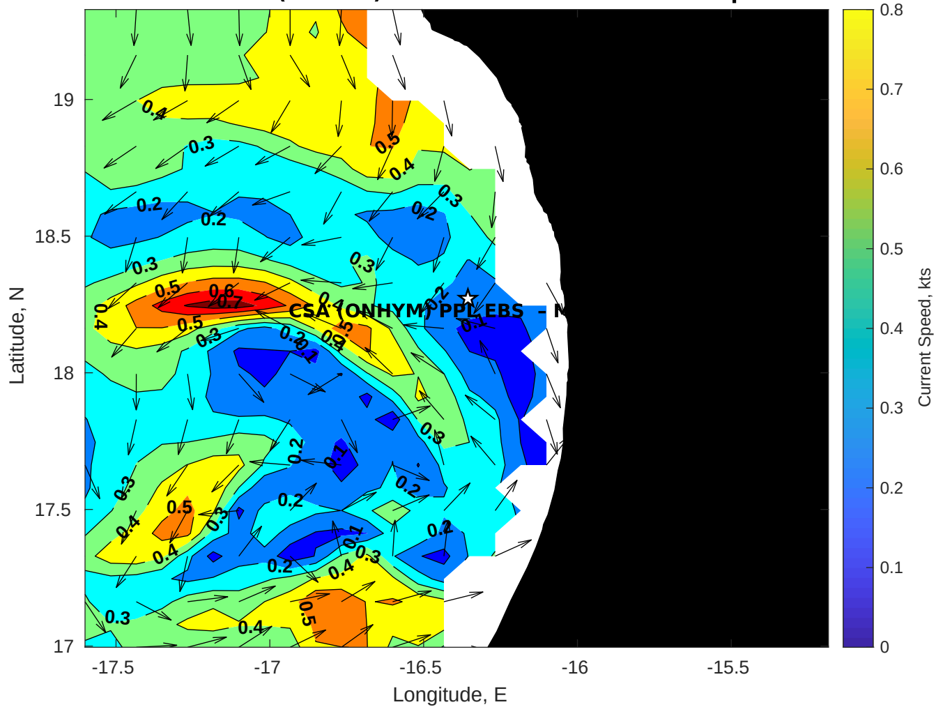
Surface Currents for CSA (ONHYM) PPL EBS - Mauritania at 29-Apr-2025 00:00:00
