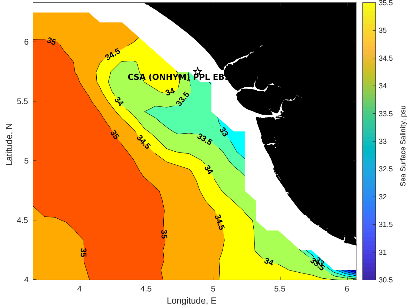
Surface Salinity for CSA (ONHYM) PPL EBS - Nigeria at 29-Apr-2025 00:00:00
