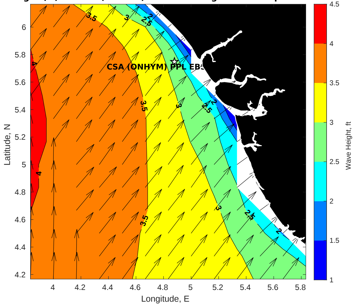
Wave Height (ft) for CSA (ONHYM) PPL EBS - Nigeria at 30-Apr-2025 09:00:00
