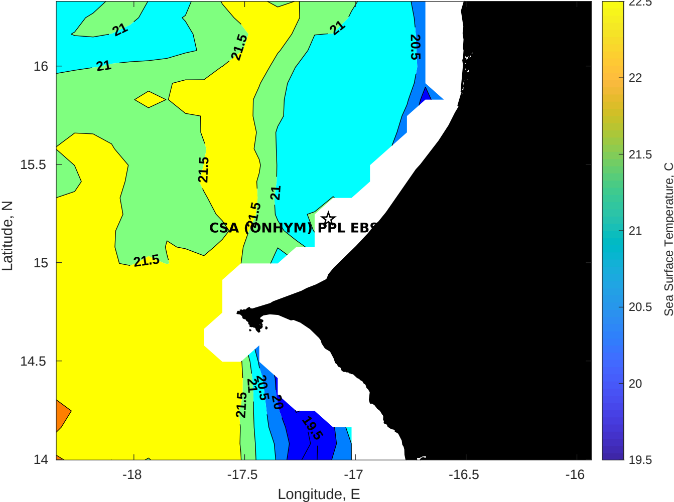
SST for CSA (ONHYM) PPL EBS - Senegal at 29-Apr-2025 00:00:00
