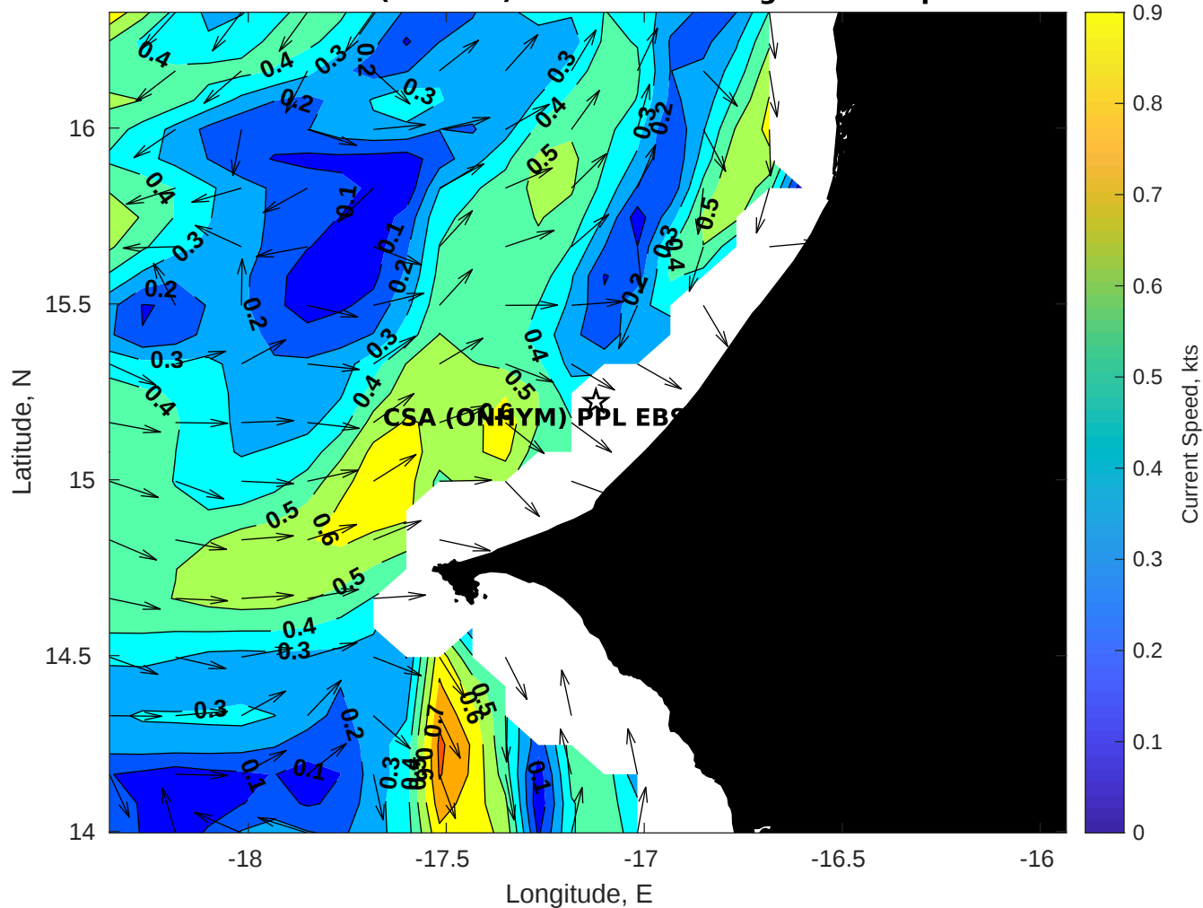
Surface Currents for CSA (ONHYM) PPL EBS - Senegal at 29-Apr-2025 00:00:00
