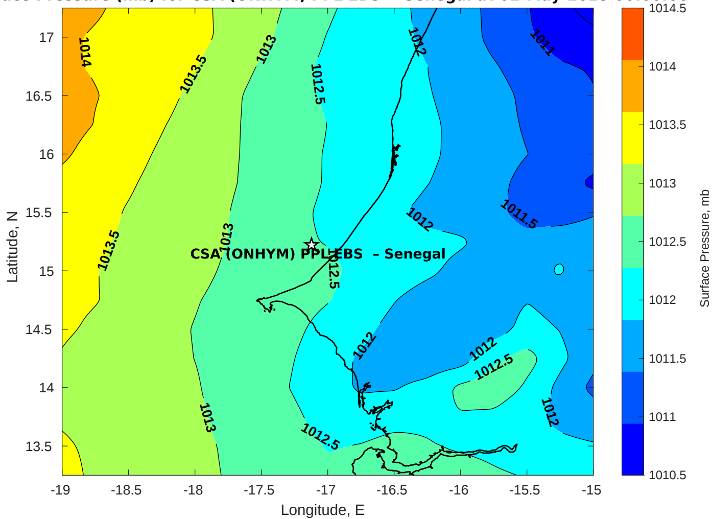
Surface Pressure (mb) for CSA (ONHYM) PPL EBS - Senegal at 02-May-2025 00:00:00
