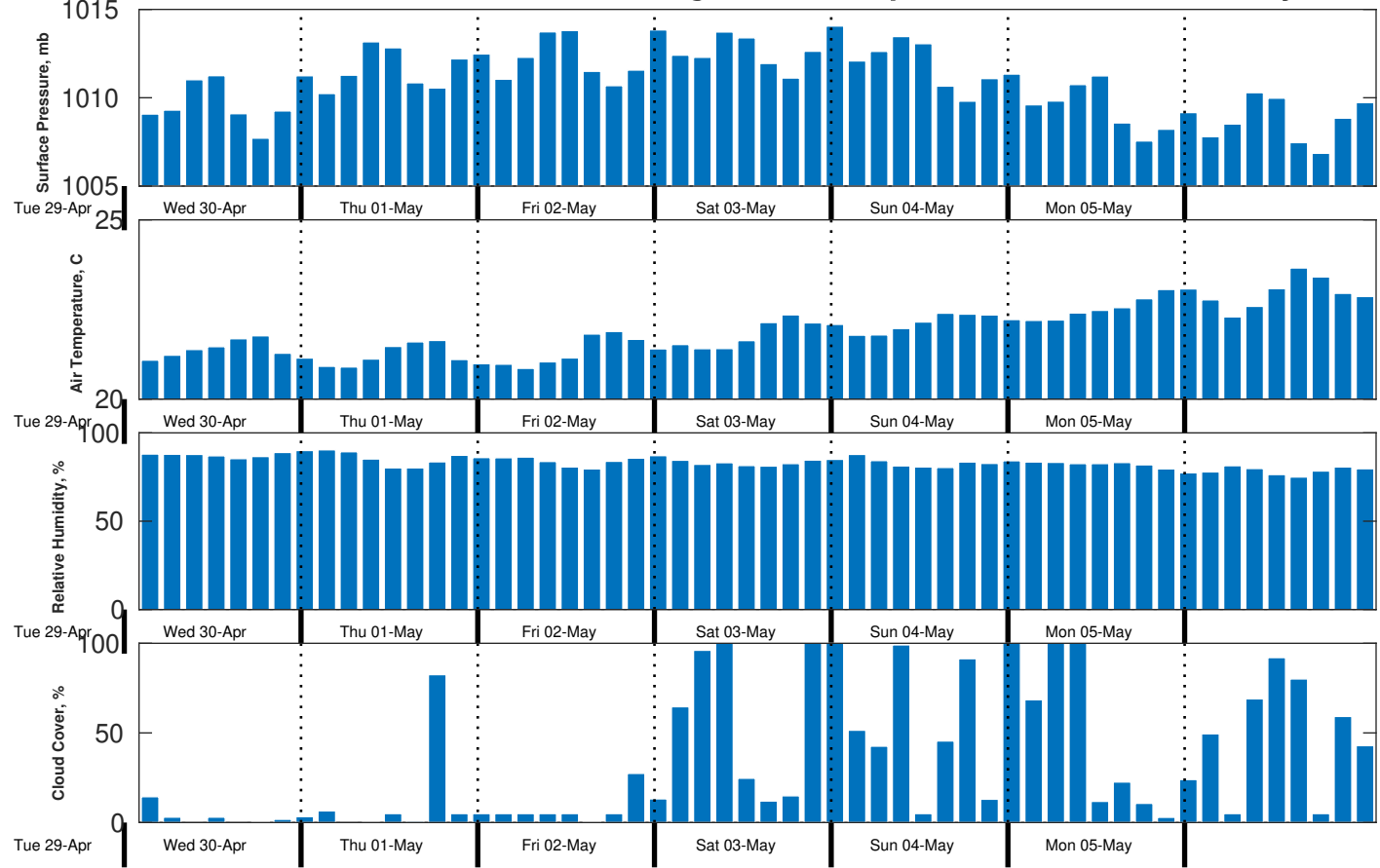
Met Forecast for CSA (ONHYM) PPL EBS - Senegal from 30-Apr-2025 00:00:00 to 07-May-2025 00:00:00
