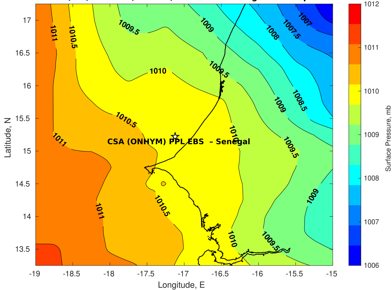
Surface Pressure (mb) for CSA (ONHYM) PPL EBS - Senegal at 30-Apr-2025 00:00:00
