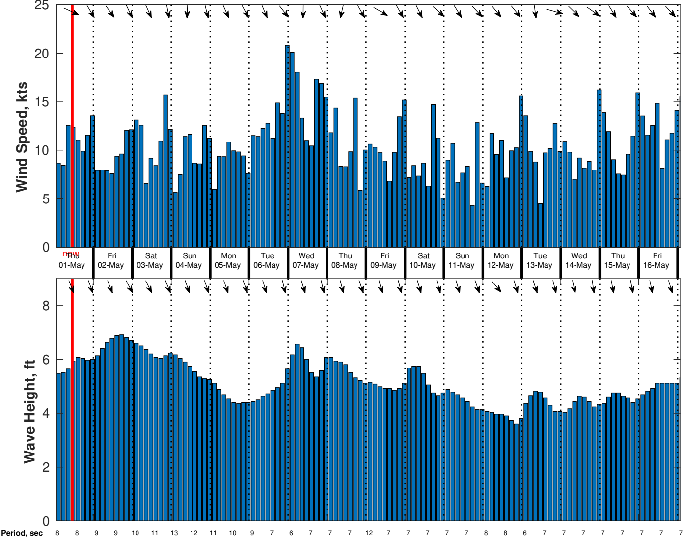
Wind & Wave Forecast for CSA (ONHYM) PPL EBS - Senegal from 30-Apr-2025 01:00:00 to 16-May-2025 01:00:00
