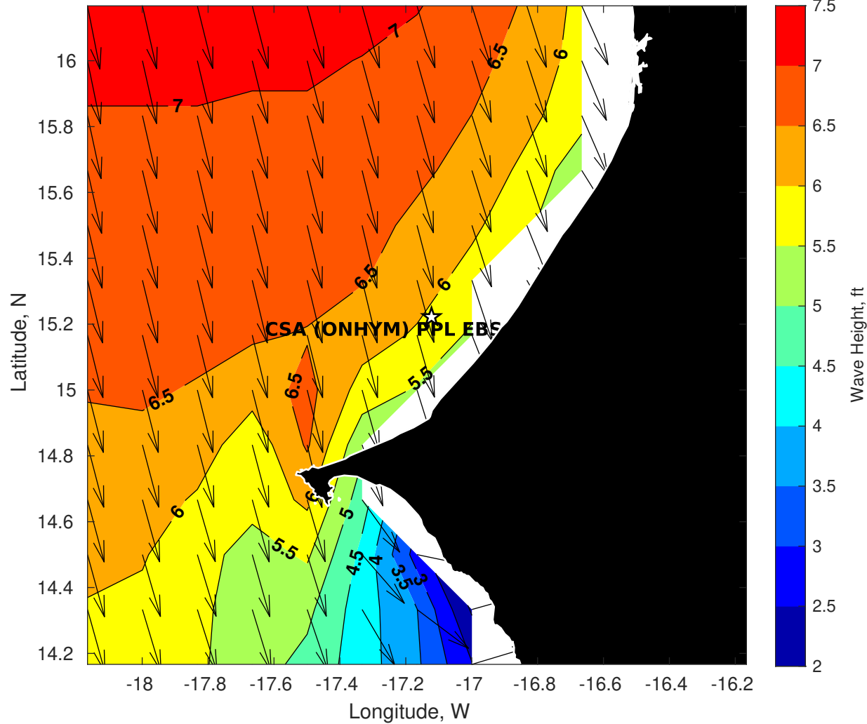
Wave Height (ft) for CSA (ONHYM) PPL EBS - Senegal at 30-Apr-2025 09:00:00
