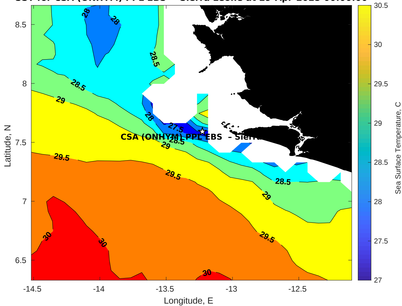
SST for CSA (ONHYM) PPL EBS - Sierra Leone at 29-Apr-2025 00:00:00
