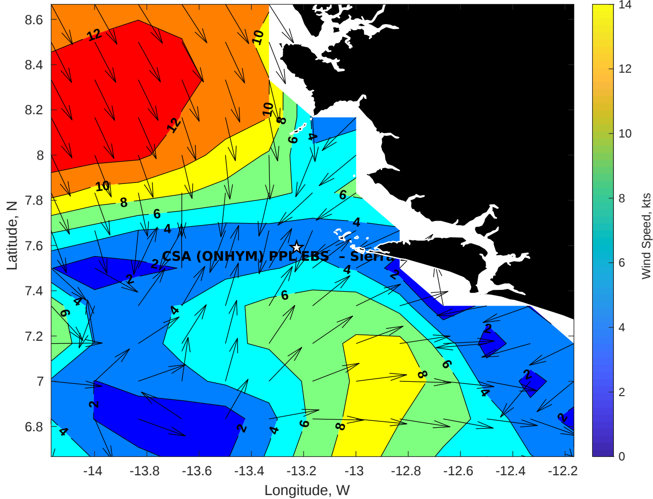
Winds (kts) for CSA (ONHYM) PPL EBS - Sierra Leone at 30-Apr-2025 09:00:00
