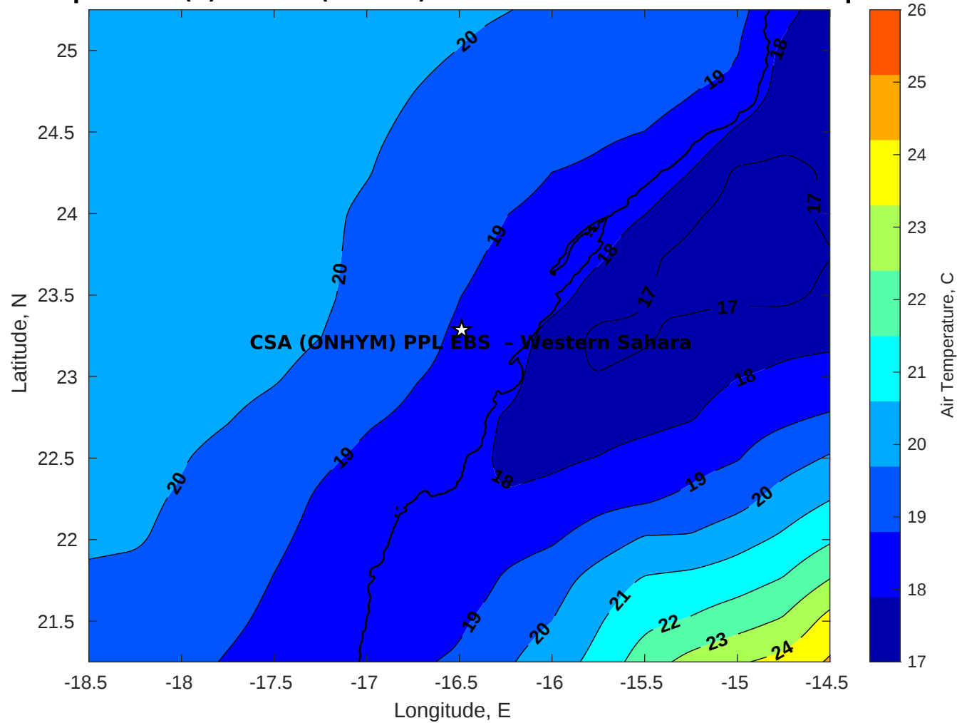
Air Temperature (C) for CSA (ONHYM) PPL EBS - Western Sahara at 30-Apr-2025
