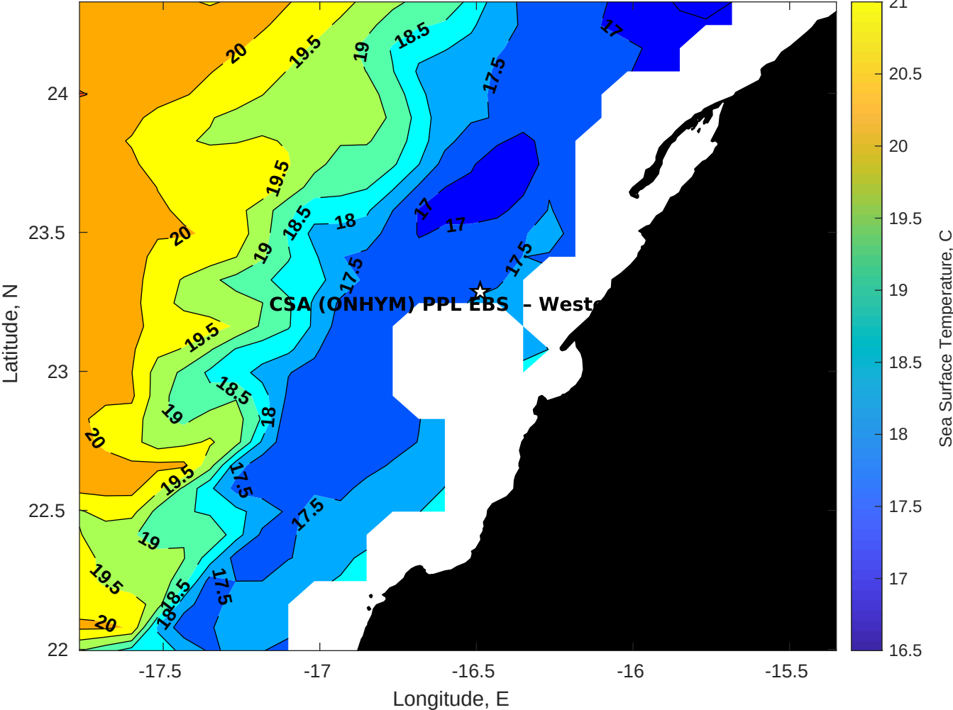
SST for CSA (ONHYM) PPL EBS - Western Sahara at 29-Apr-2025 00:00:00
