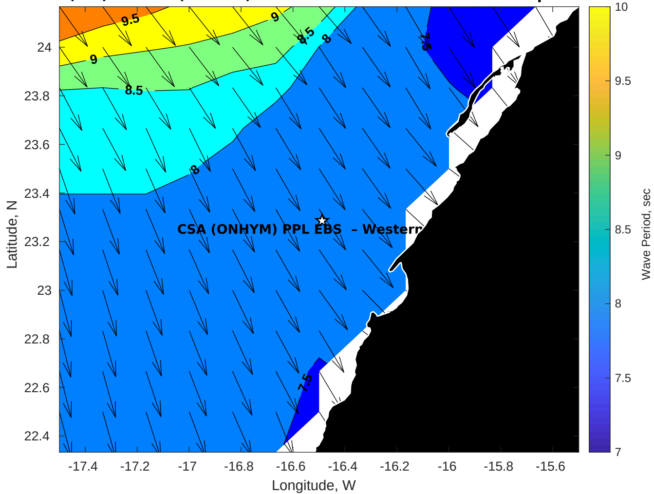
Wave Period (sec) for CSA (ONHYM) PPL EBS - Western Sahara at 30-Apr-2025 09:00:00
